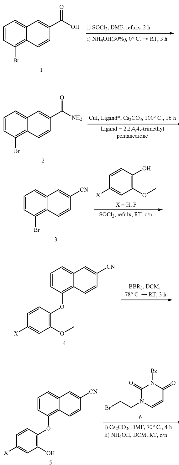
Scheme 4. Synthesis of the Naphthalene Inhibitors
