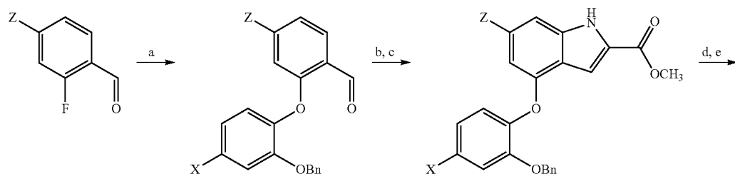
Scheme 1. Synthesis of the 2-Cyanoindoles
