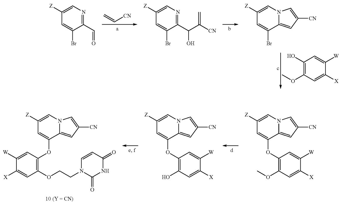
Scheme 2. Synthesis of the 2-Cyanoindolizines
