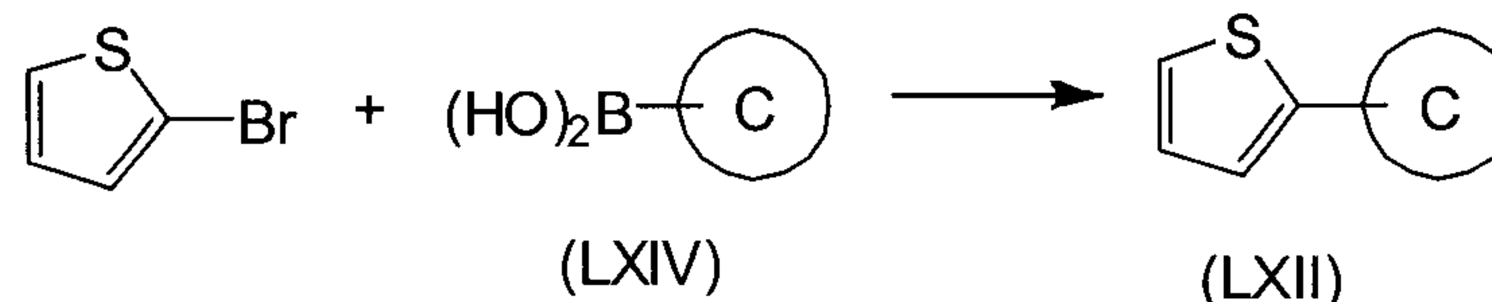
Scheme 10
