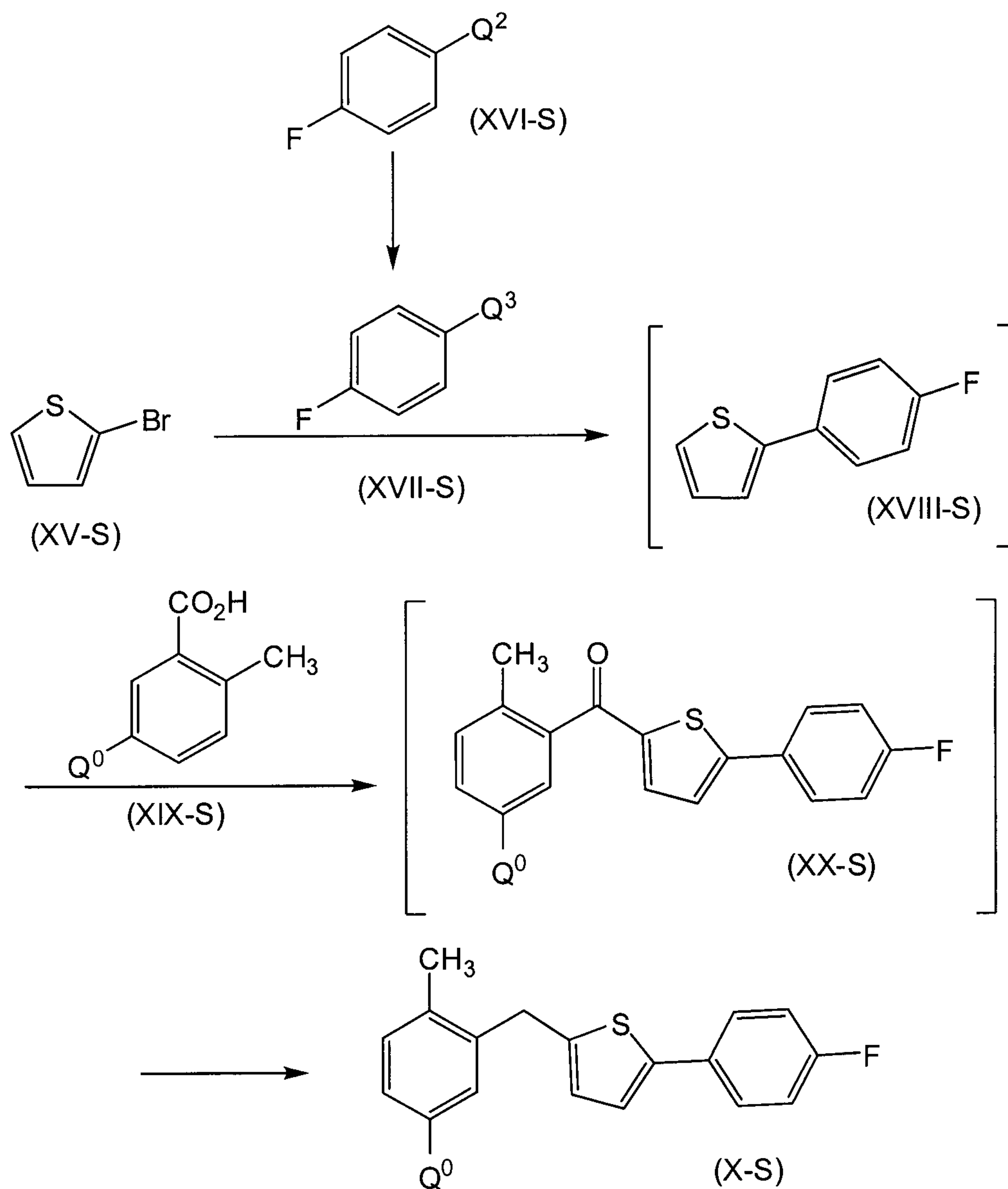
Scheme 4
