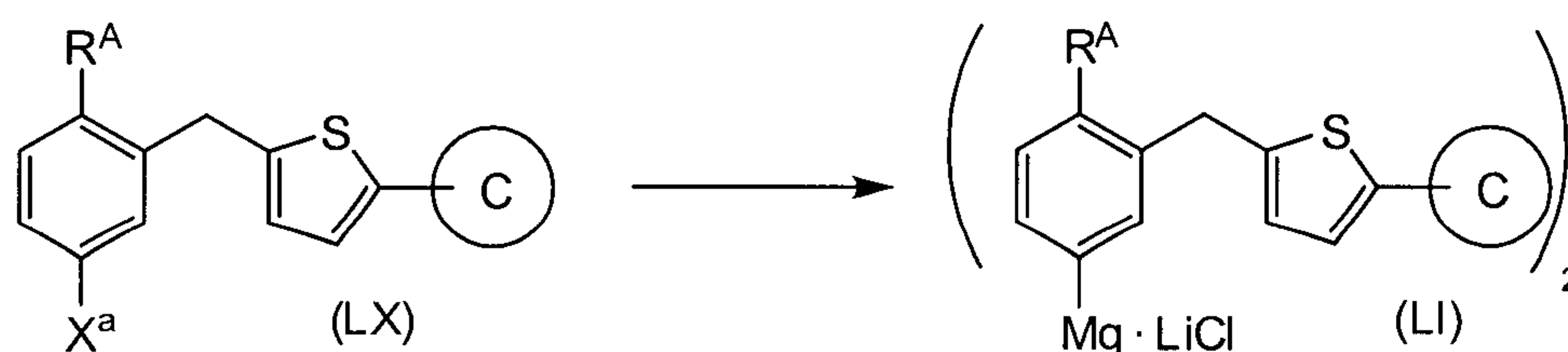
Scheme 8
