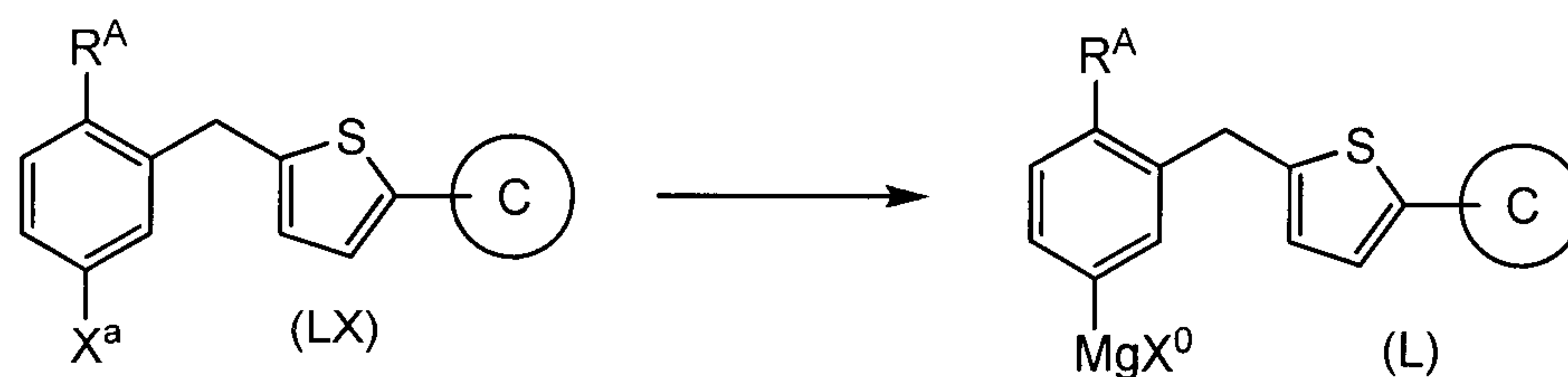
Scheme 7
