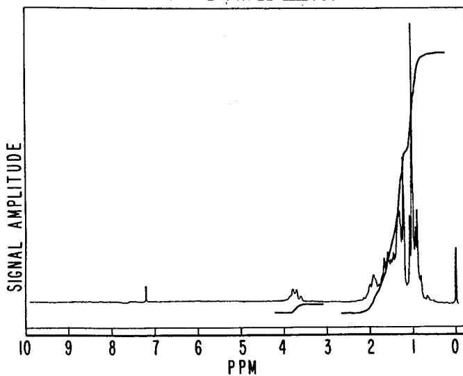
N M R SPECTRUM FOR EXAMPLE VII(B).
