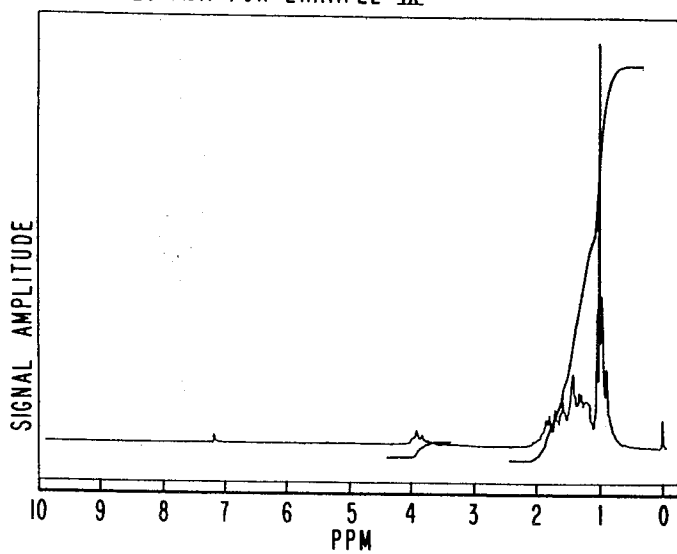
NMR SPECTRUM FOR EXAMPLE IX
