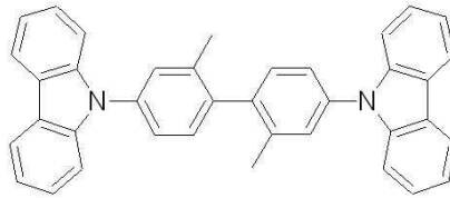
dmCBP
