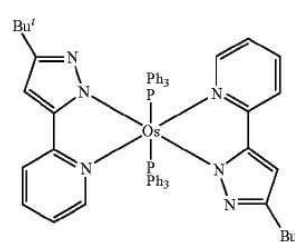
Os(bppz) 2 (PPh 3 ) 2
