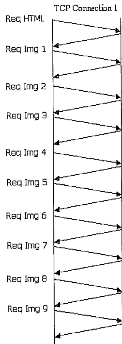
HTTP/1.1 persistent connection
