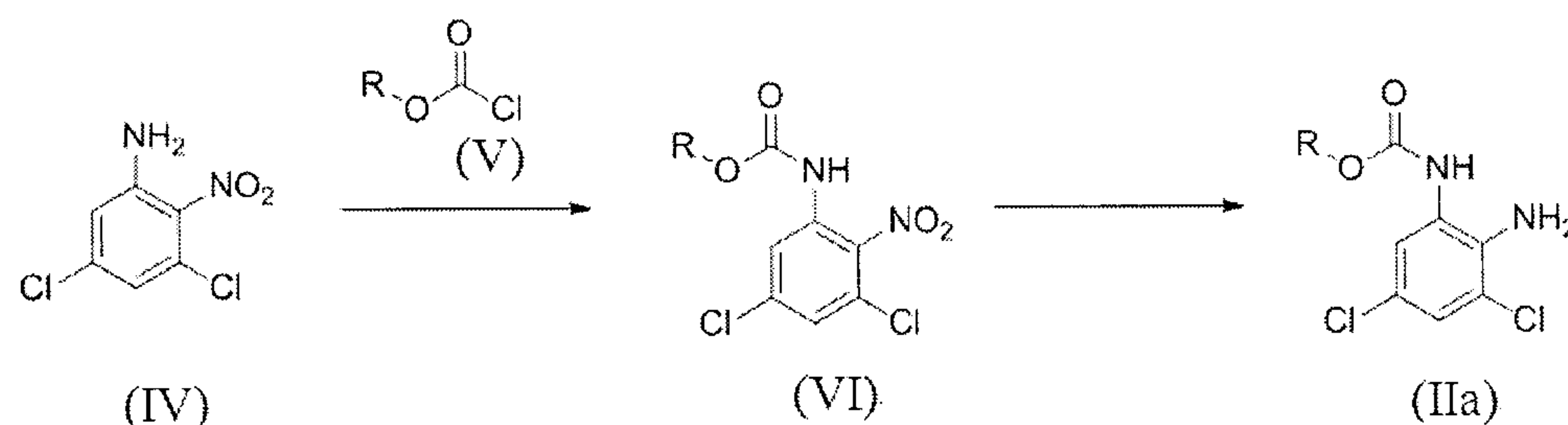
[Reaction Scheme 2]
