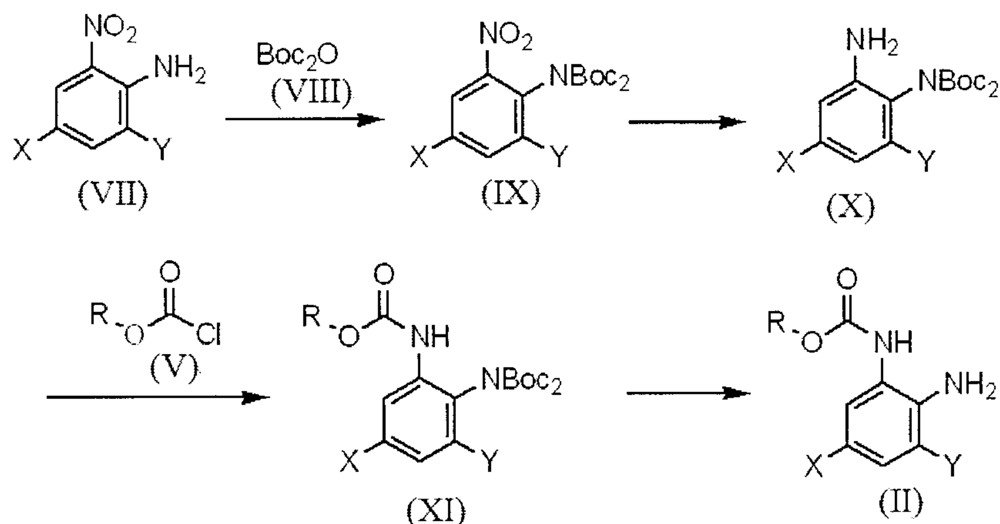
[Reaction Scheme 3]
