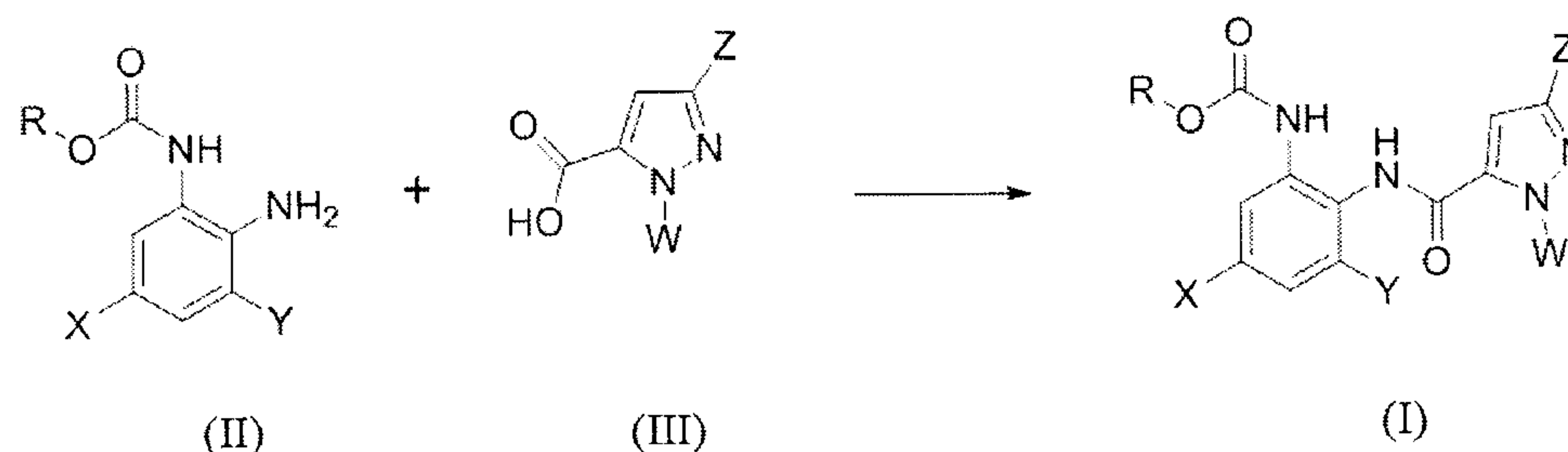
[Reaction Scheme 1]
