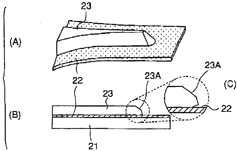
FIG. 3 PRIOR ART
