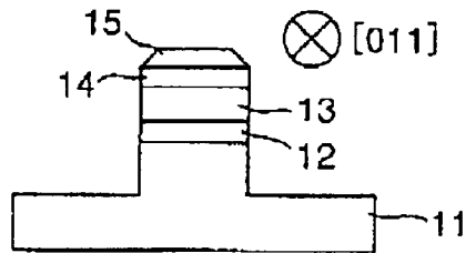
FIG. 1C PRIOR ART
