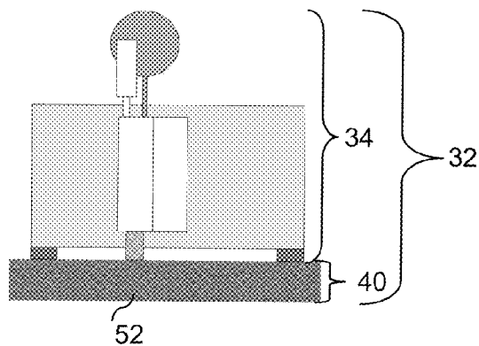
FIG. 3C (PRIOR ART)
