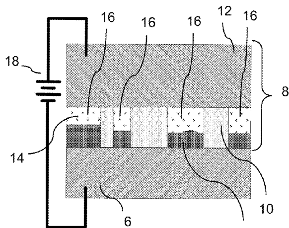
FIG. 2A (PRIOR ART) 4
