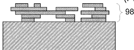
FIG. 4I (PRIOR ART)
