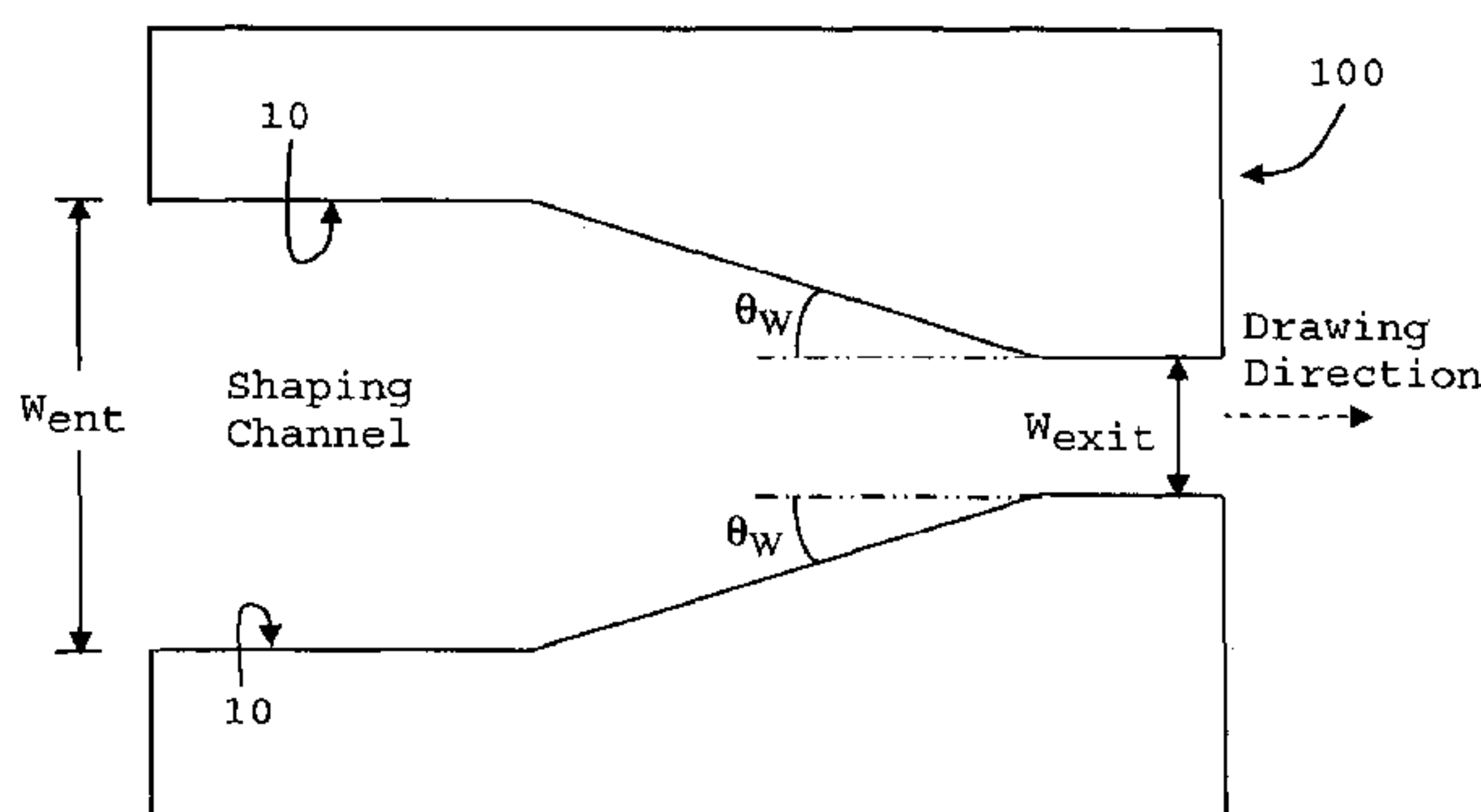
B Cut-away view down height dimension of a Proportional Die.
