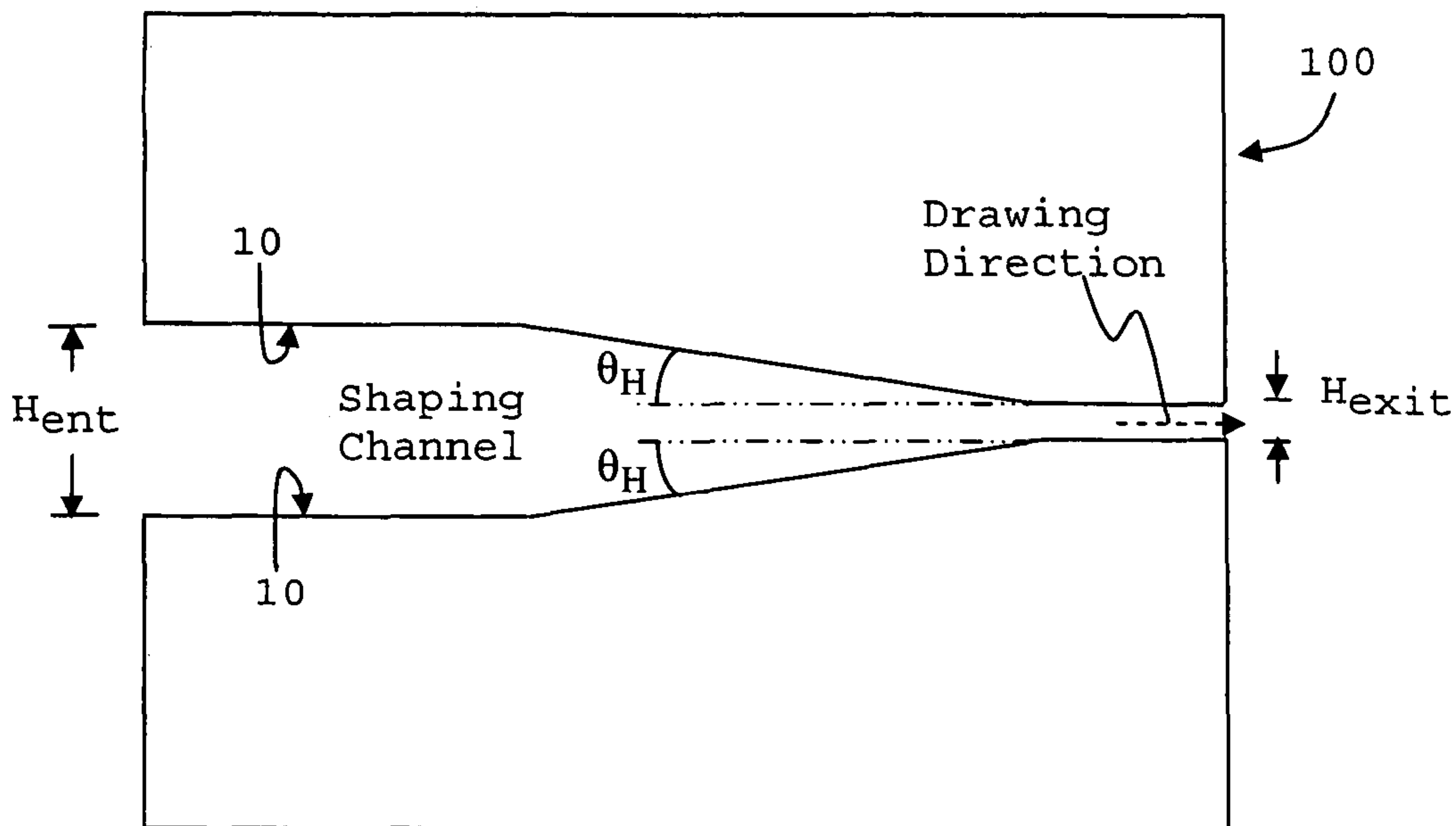
A Cut-away view down width dimension of a Proportional Die.
