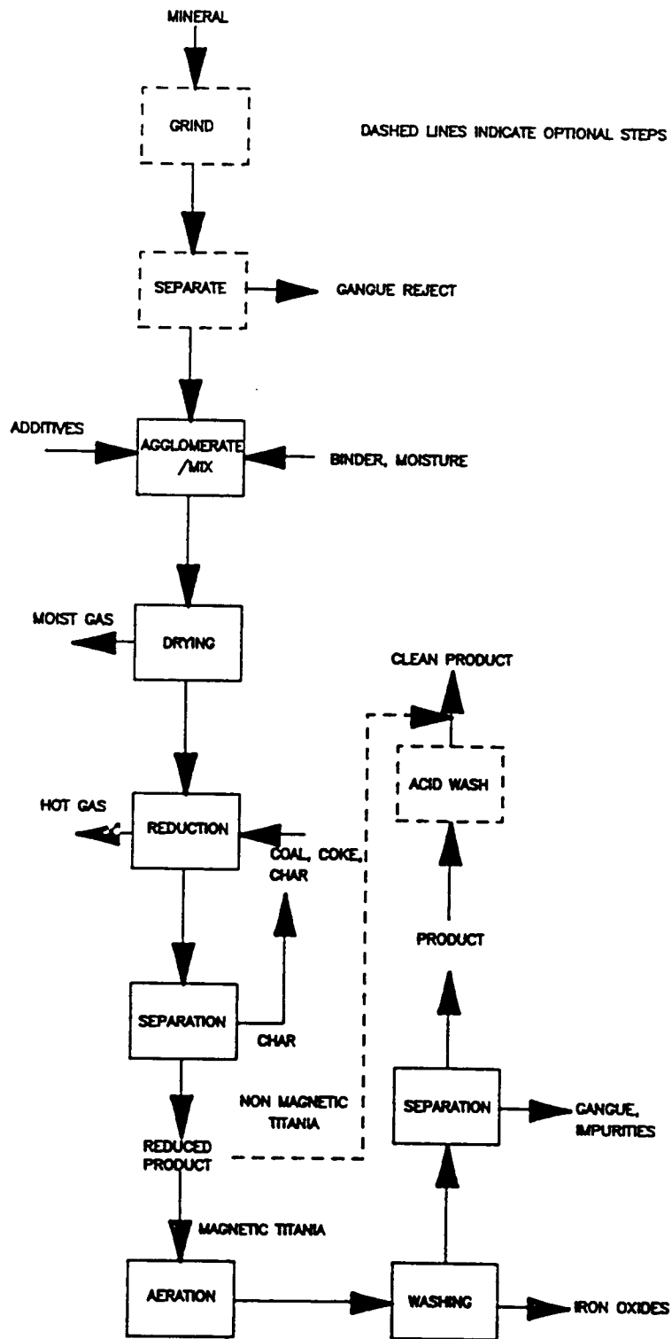
FIGURE 1: FLOWSHEET OF PROCESS FOR PRODUCING ACID SOLUBLE TITANIA
