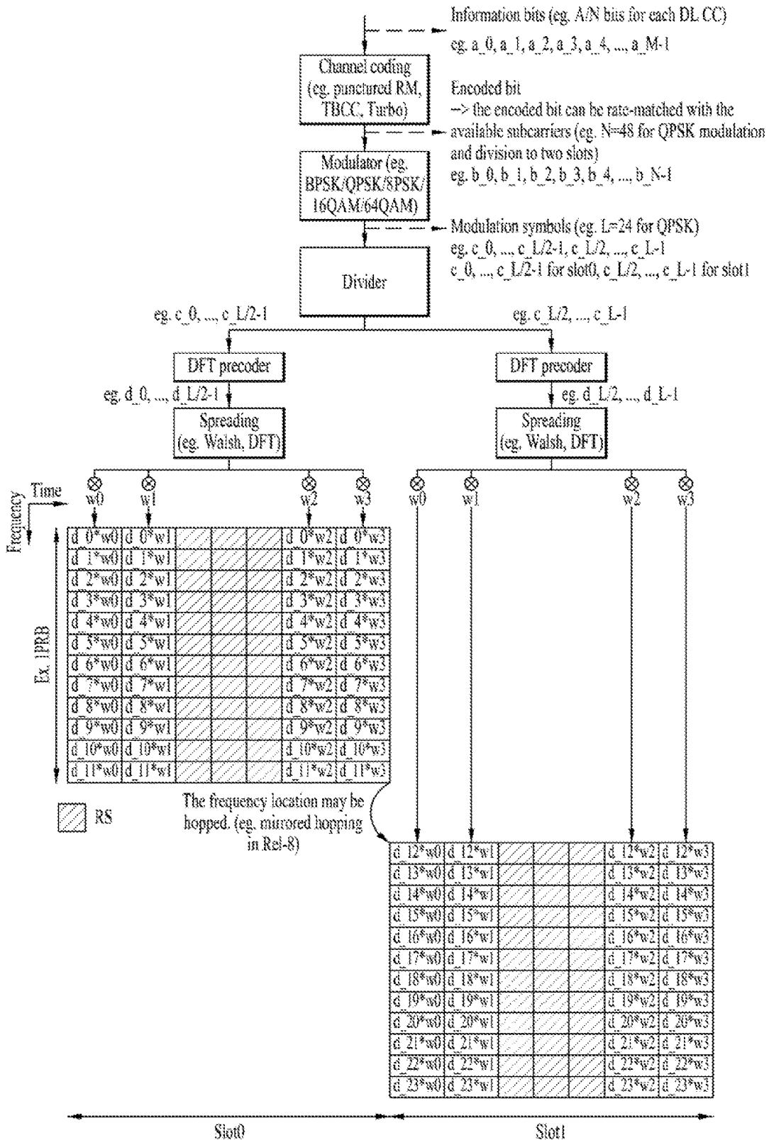
Reuse of LTE PUCCH Format 1 structure (Normal CP case)
