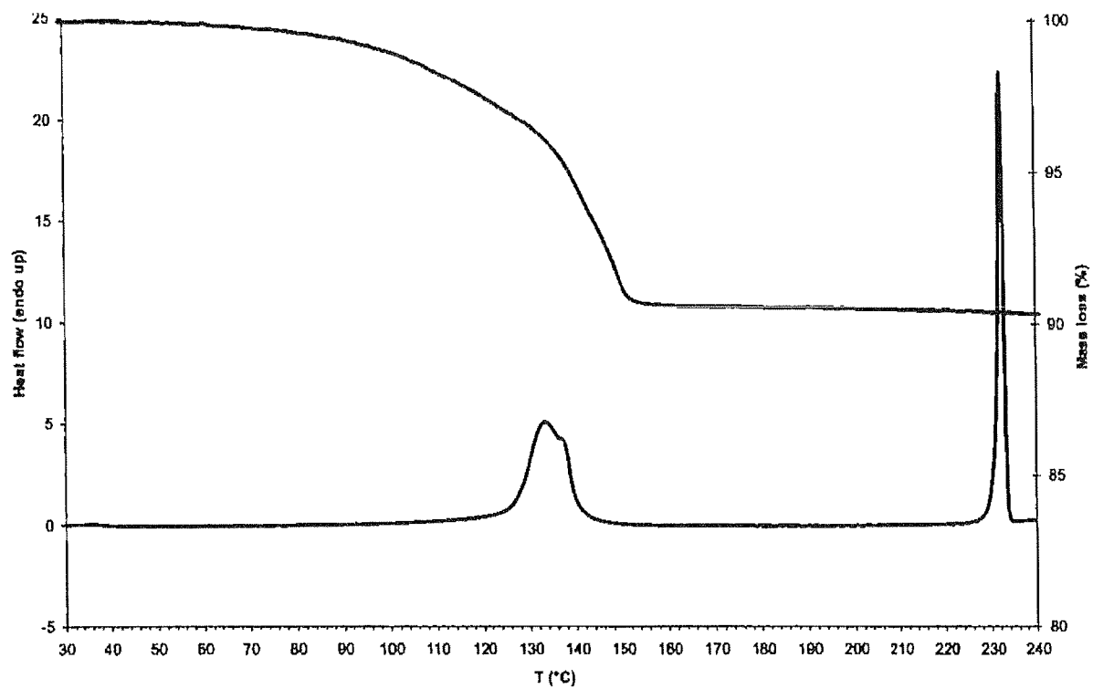
DSC (lower curve; left ordinate), and TGA (upper curve; right ordinate) curves of formic acid solvate of Rivaroxaban
