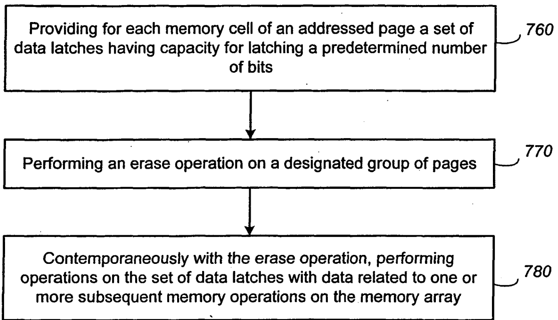
Cache Operation During Erase Operation
