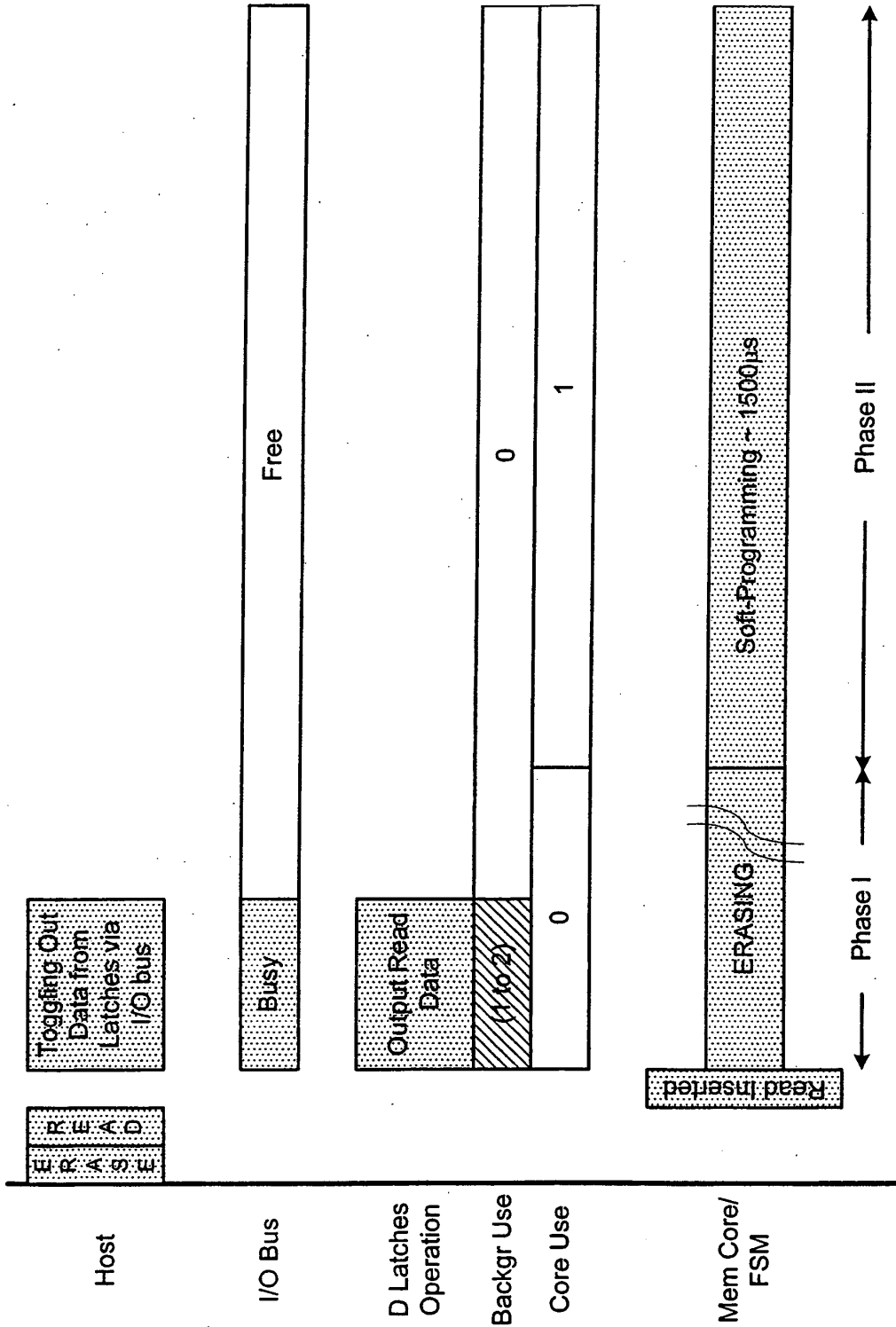
PREEMPTIVE BACKGROUND READ DURING ERASE
