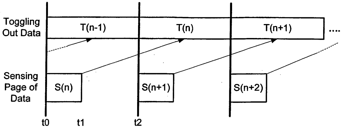
Conventional Read Caching FIG. 37
