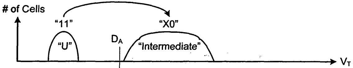
Lower Page Programming (LM Gray Code)
