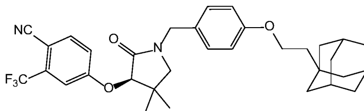
Compound 51
