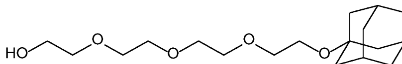
Compound 12
