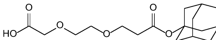
Compound 23
