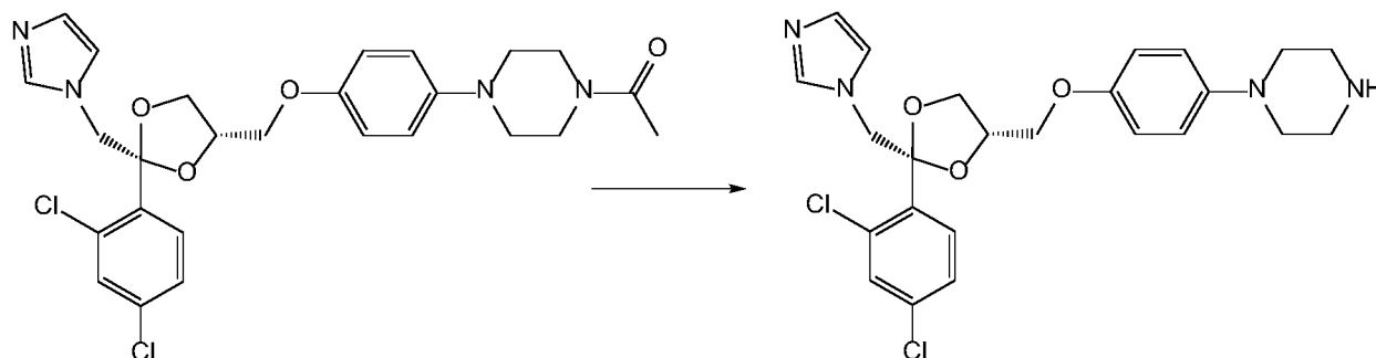
Scheme 13
