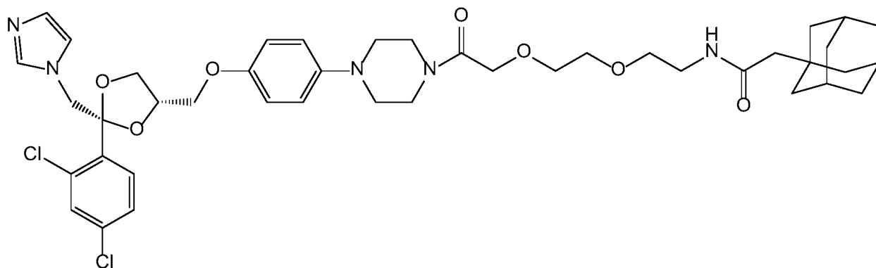
Compound 42
