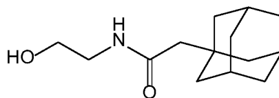
Compound 1
