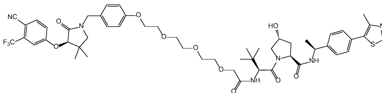
Compound 54
