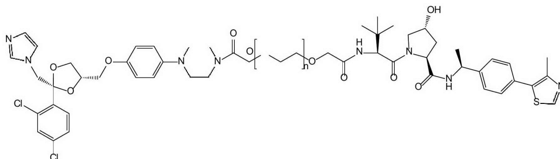
(XXIII)
