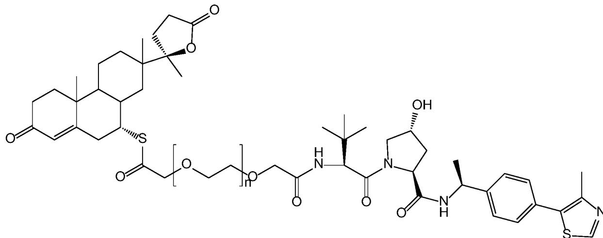
Scheme 18
