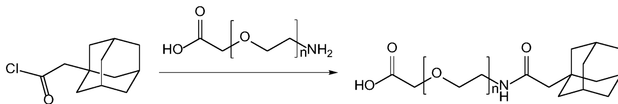
Scheme 4
