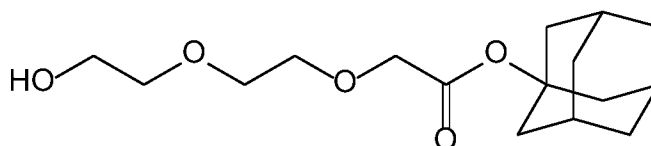
Compound 31
