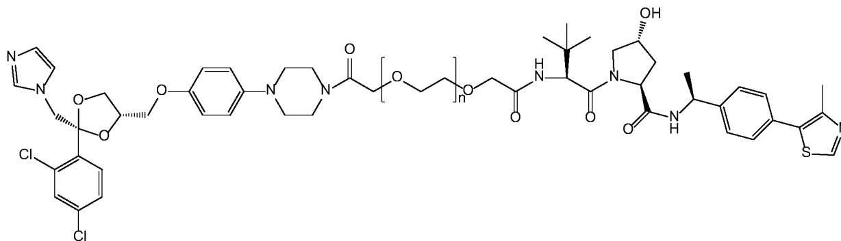
Scheme 19
