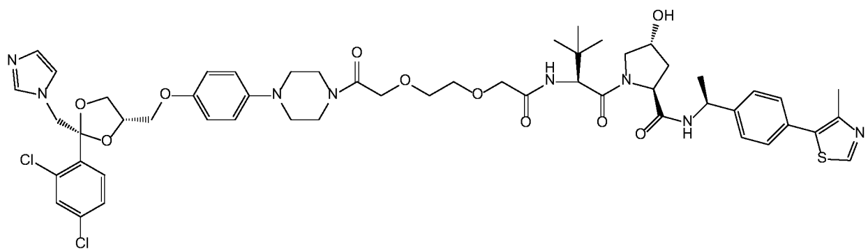
Compound 48
