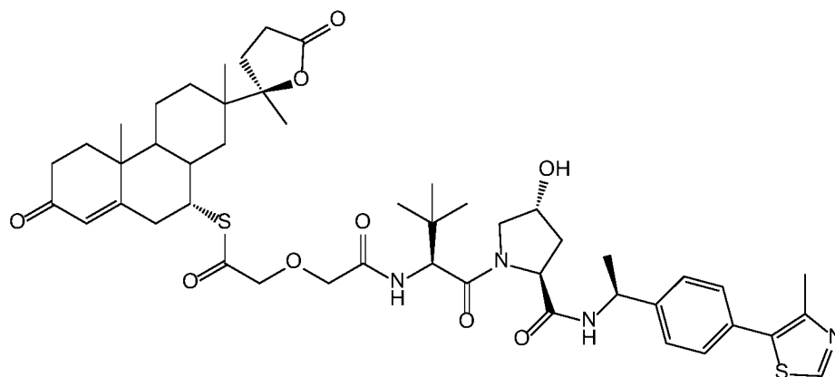
Compound 43
