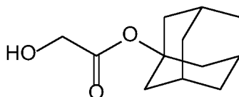
Compound 29
