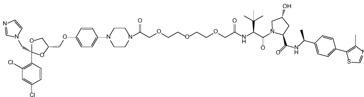
Compound 49
