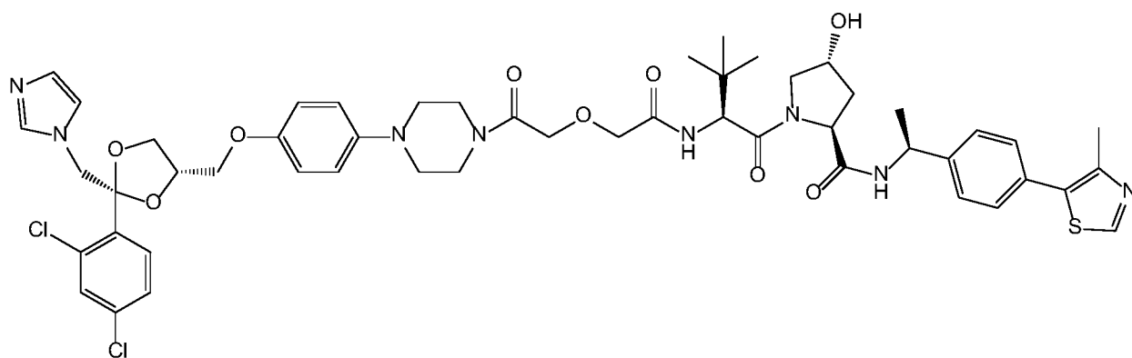
Compound 47
