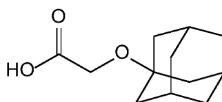
Compound 13
