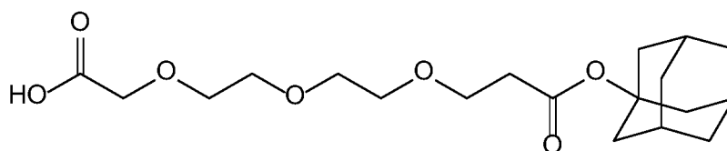
Compound 24
