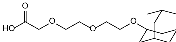
Compound 15
