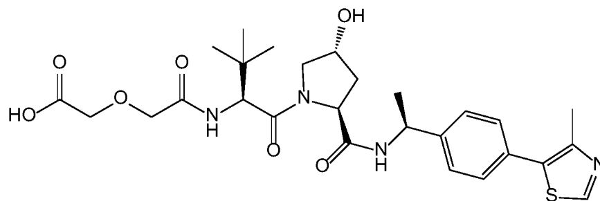
Compound 33
