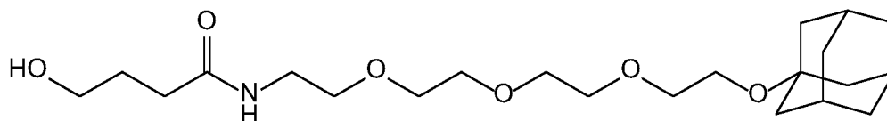
Compound 20
