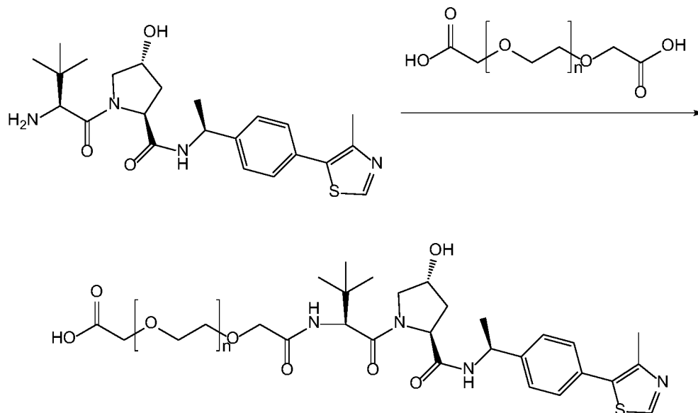
Scheme 11
