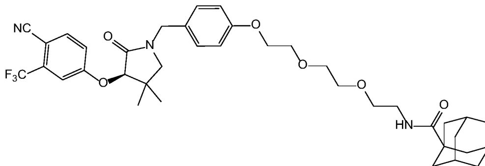
Compound 52
