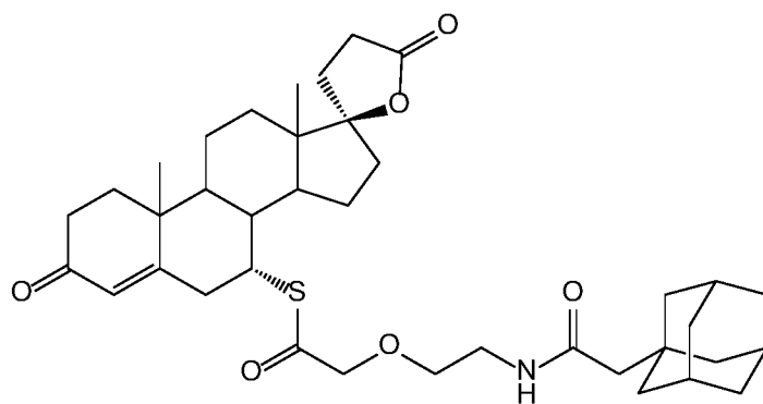
Compound 38
