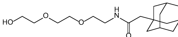
Compound 3
