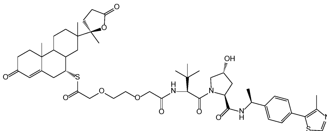
Compound 44
