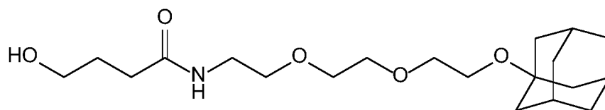
Compound 19
