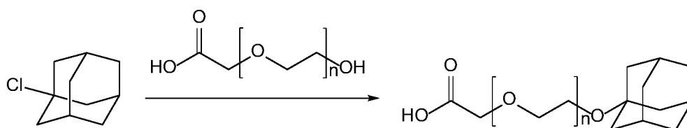
Scheme 6
