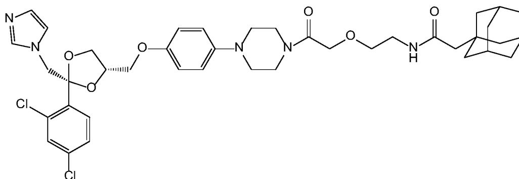
Compound 41
