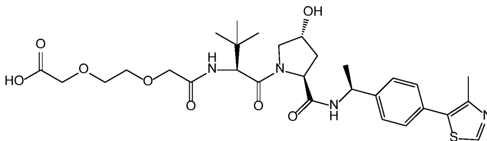
Compound 34
