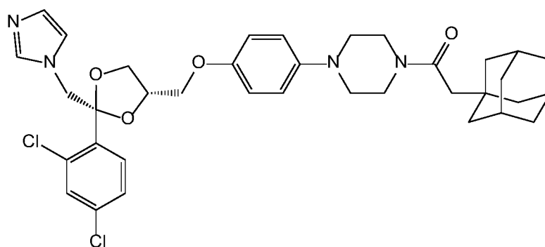
Compound 40
