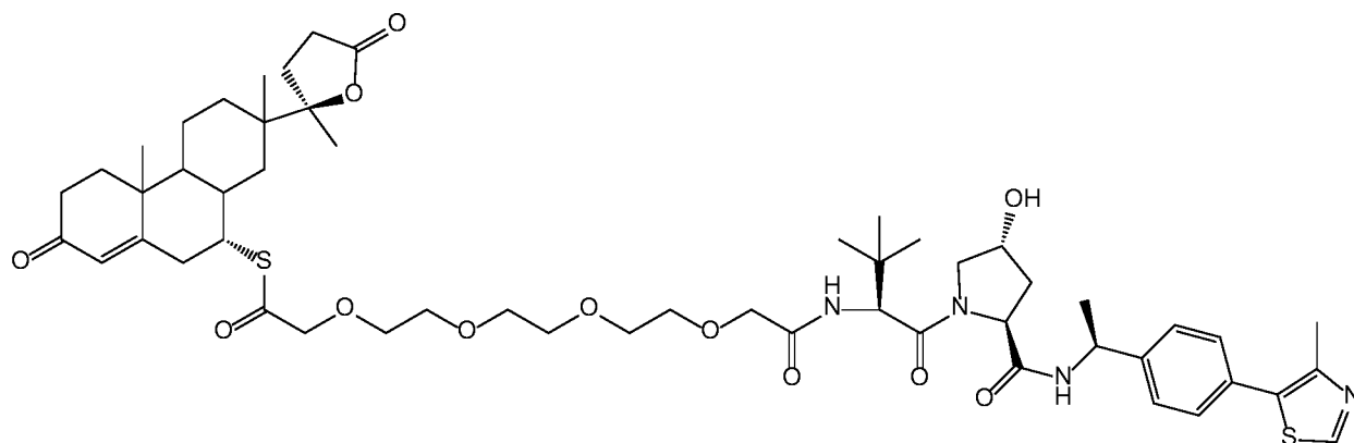
Compound 46
