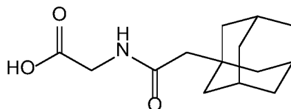
Compound 5
