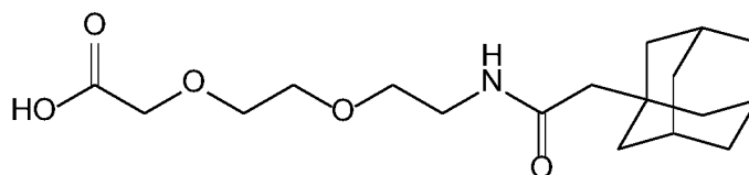
Compound 7
