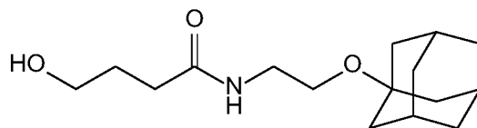
Compound 17
