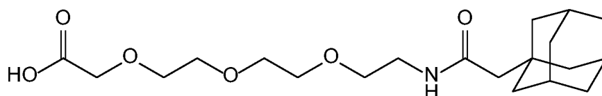
Compound 8
