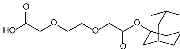
Compound 26
