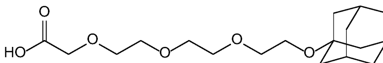
Compound 16
