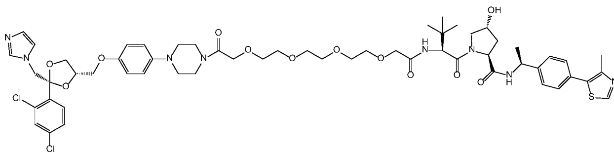
Compound 50
