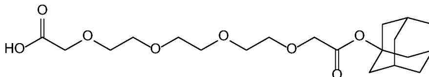
Compound 28
