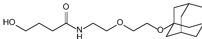
Compound 18
