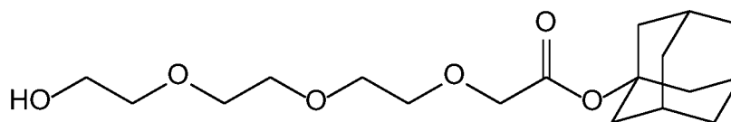
Compound 32
