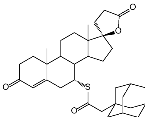
Compound 37
