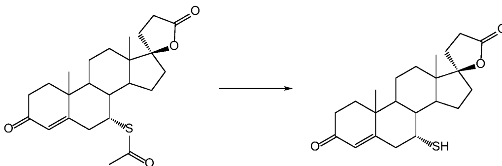
Scheme 12
