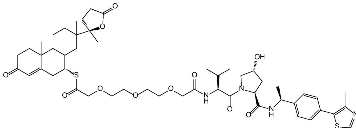
Compound 45
