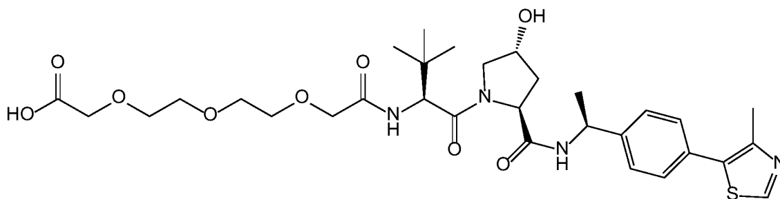
Compound 35
