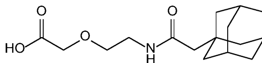
Compound 6
