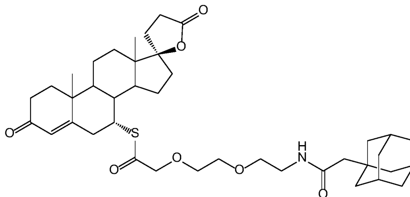
Compound 39
