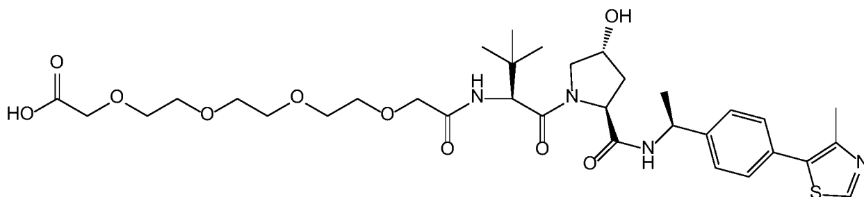
Compound 36
