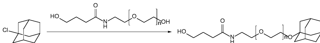
Scheme 7
