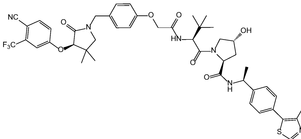
Compound 53
