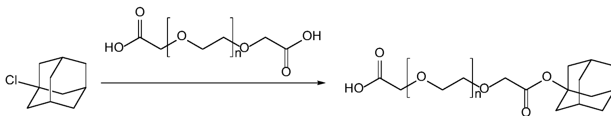
Scheme 9
