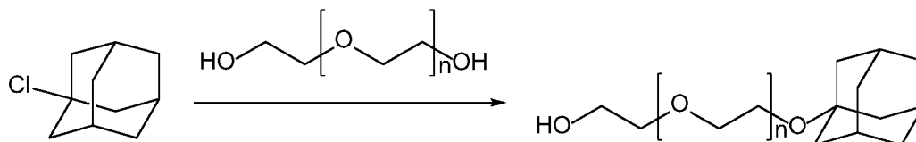
Scheme 5
