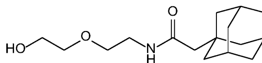
Compound 2
