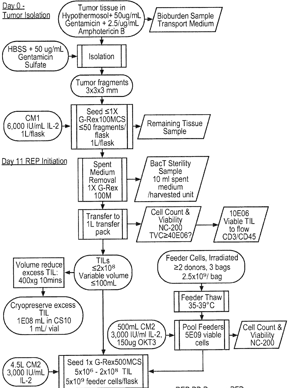
REP PD Process PFD Page 1/3 Figure 28a
