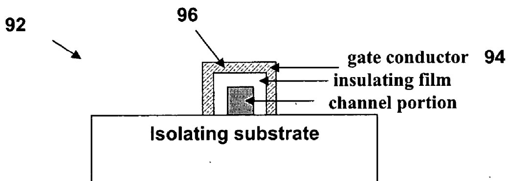
FIG. 8F (Y-Y view)
