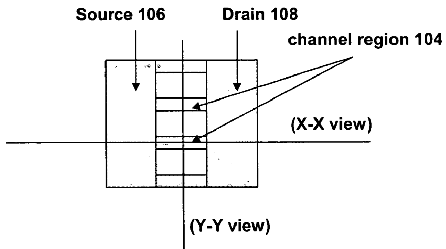
FIG. 8B (top view)
