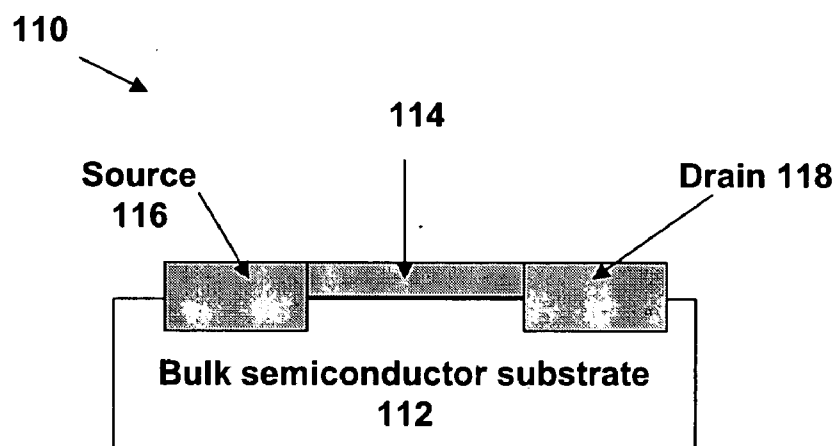
FIG. 9B (X-X view)
