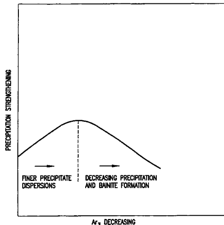
EFFECT OF FERRITE TRANSFORMATION TEMPERATURE (Ar 3 ) ON THE CONTRIBUTION FROM PRECIPITATION STRENGTHENING (ΔYS p )
