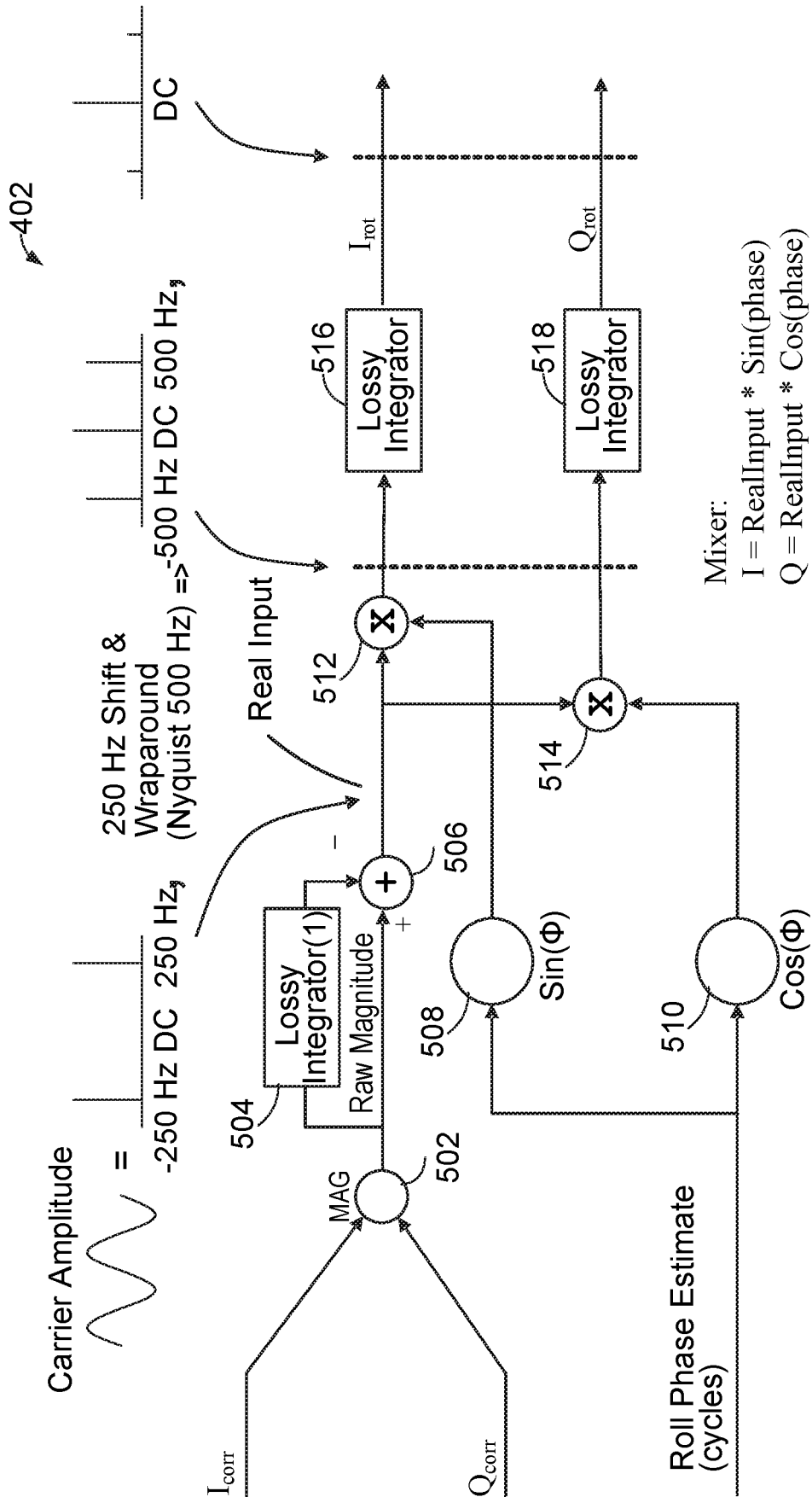
FIG. 5 Phase Rotator / Mixer
