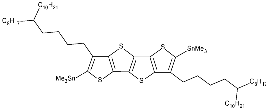
bis-trimethylstannyl-DC5BC8C10FT4
