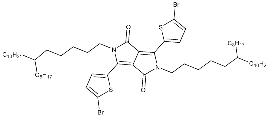
DBrTDC6BC8C10DPP
