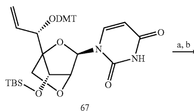
Scheme 8
