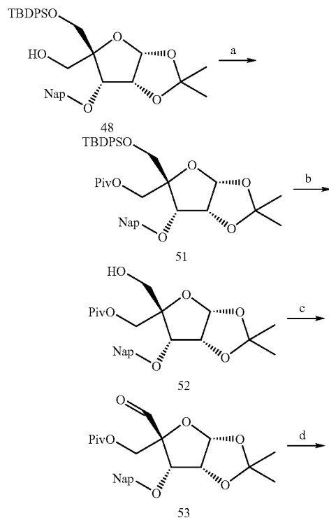
Scheme 6
