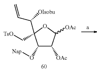
Scheme 10
