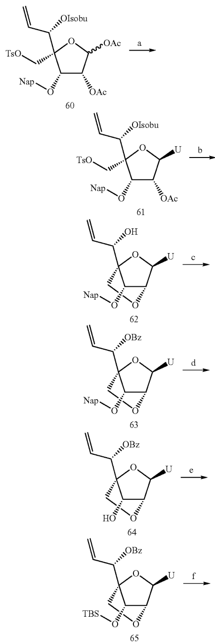
Scheme 7
