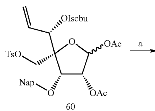
Scheme 9
