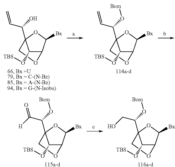
Scheme 13
