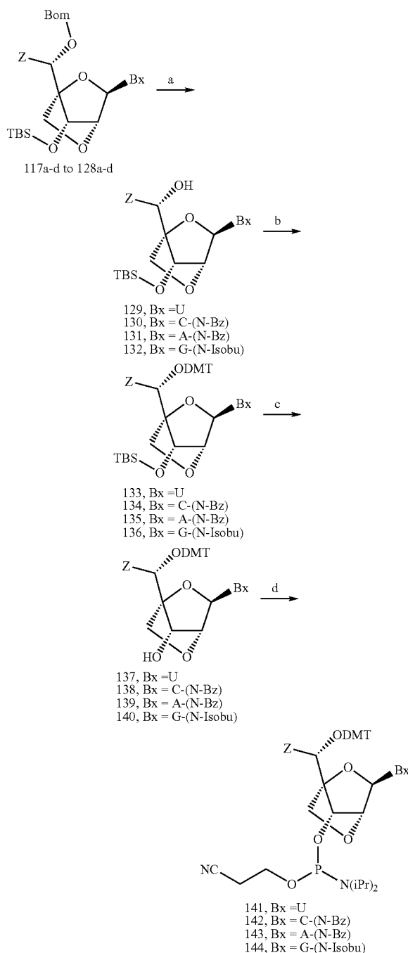
Scheme 15
