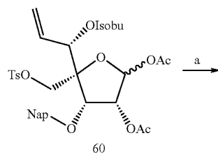
Scheme 11
