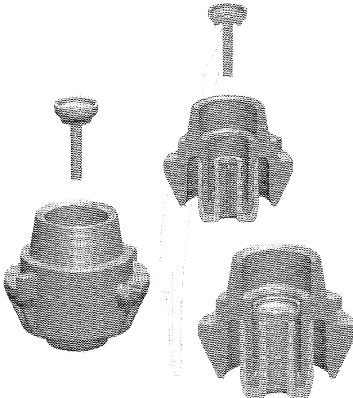
Fig. 24 - Air Valve in Power Connector
