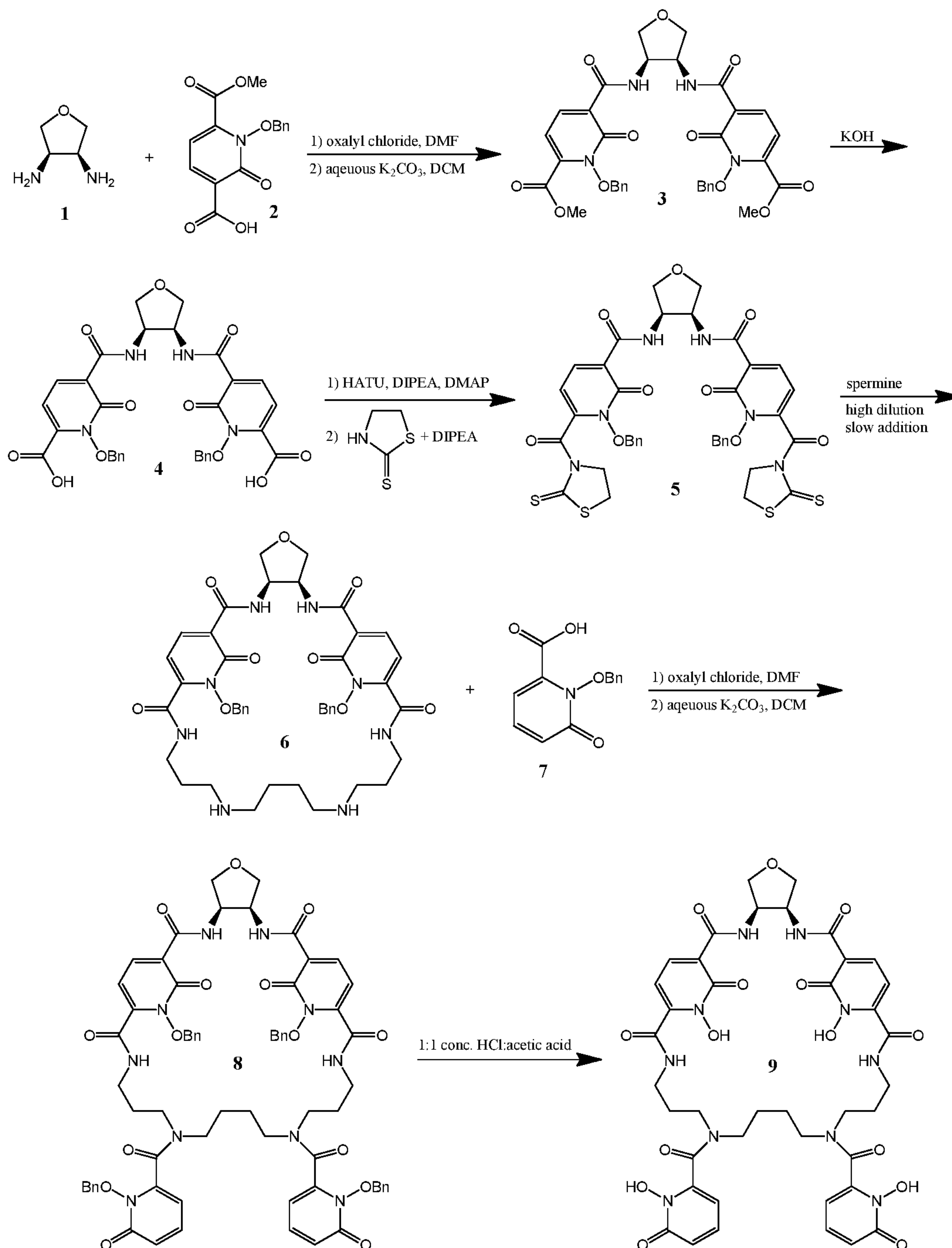
Scheme 1. Synthetic scheme for parent compound 9
