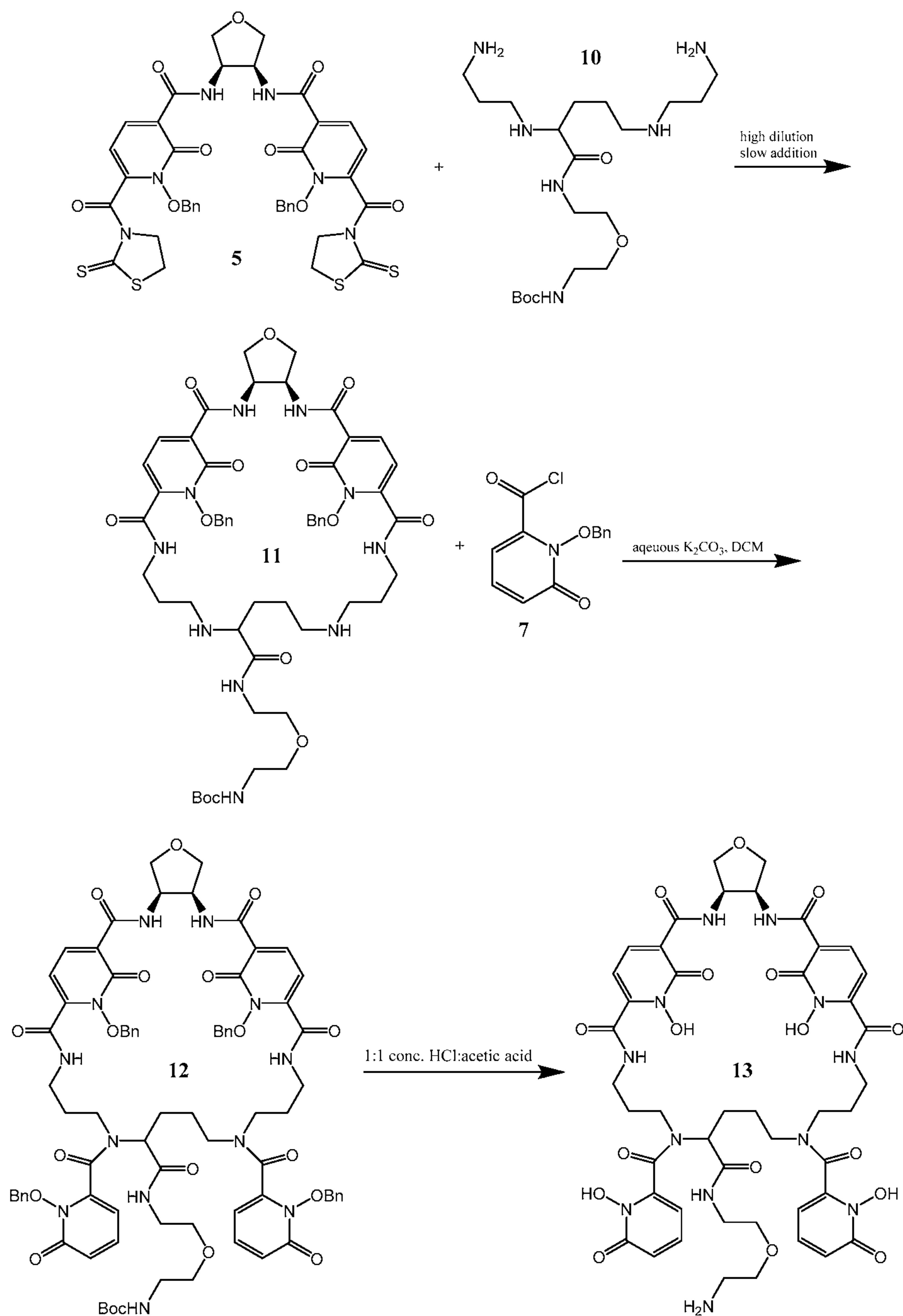
Scheme 2. Synthetic scheme for attachment point containing compound 13
