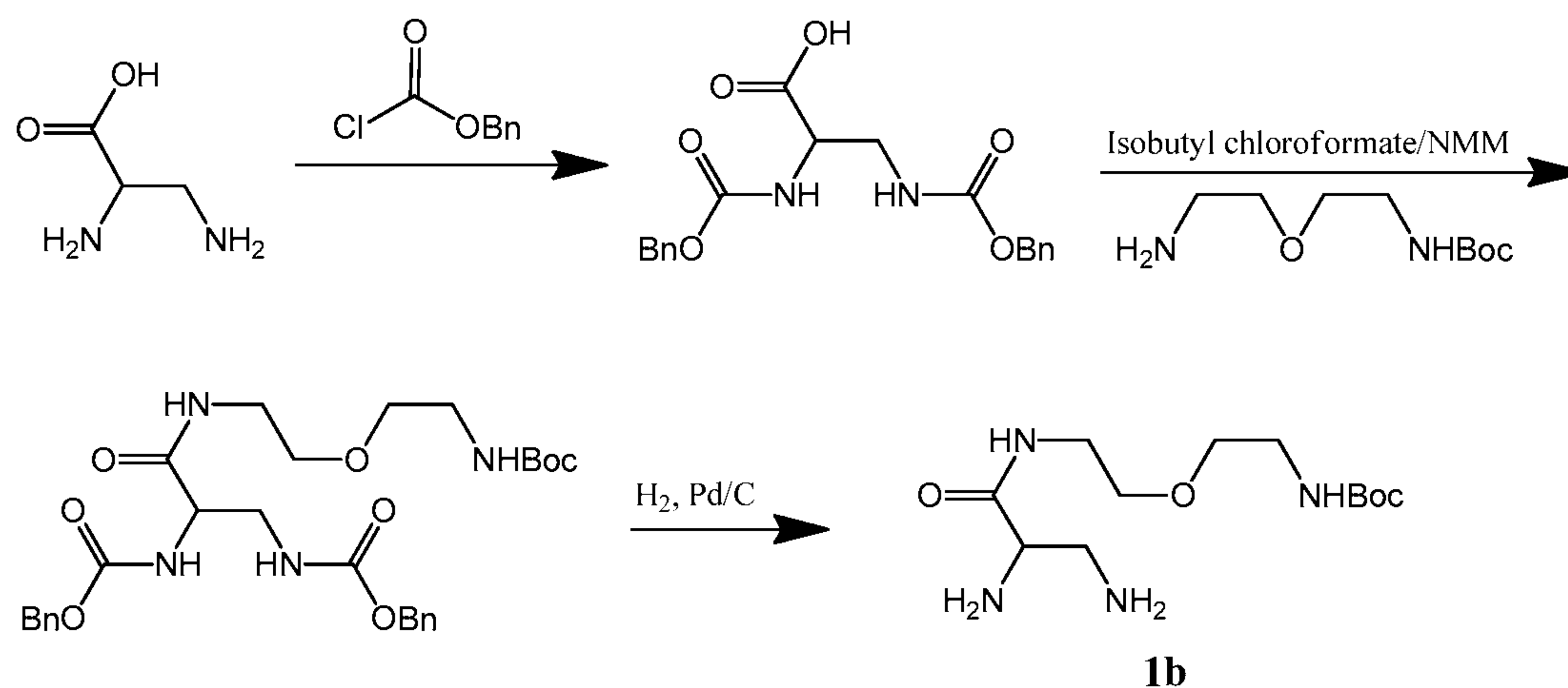
Scheme 6. Representative synthetic scheme of compound 1b .
