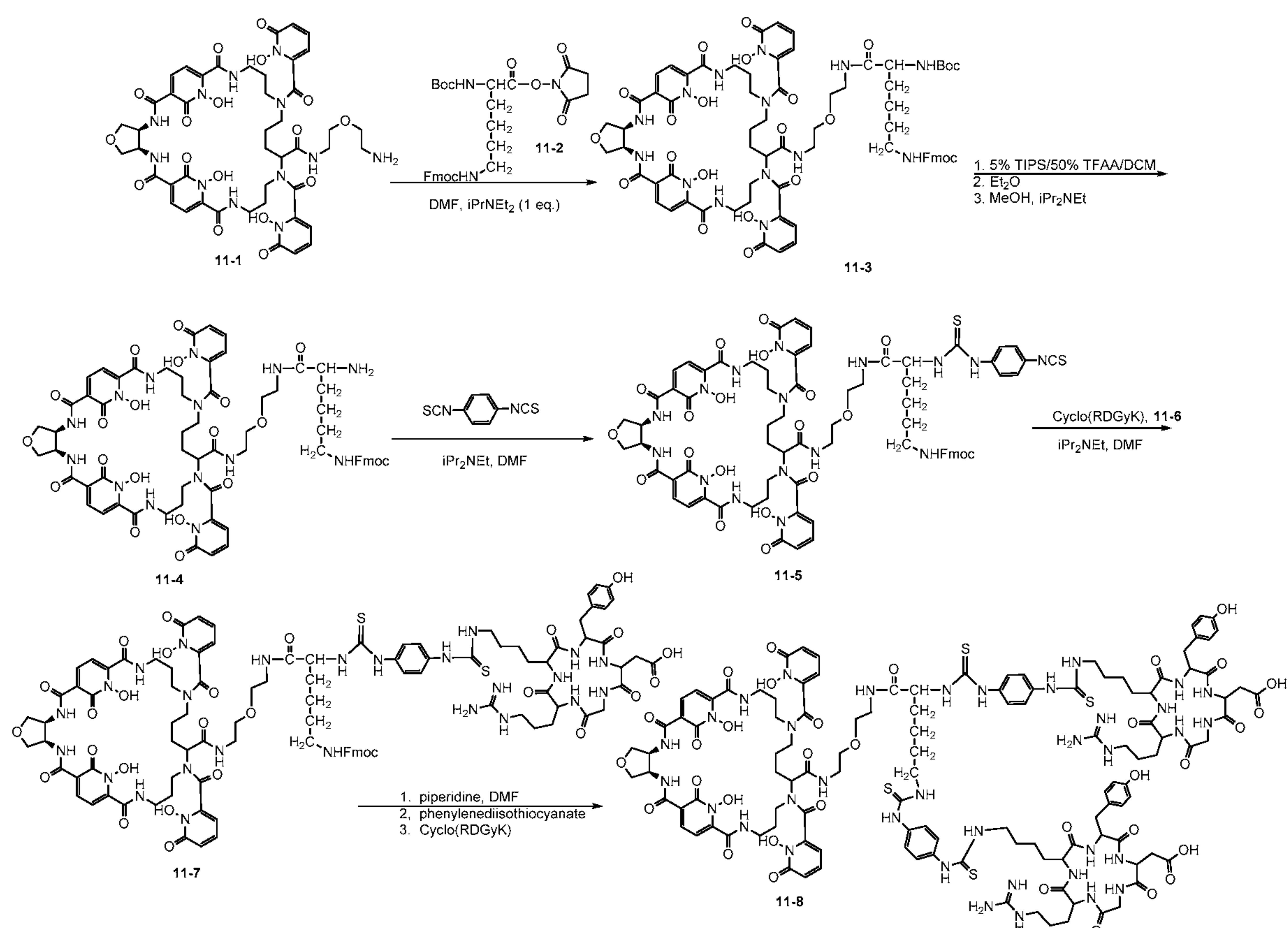
Scheme 5. Representative synthetic scheme of HOPO-Lys-cyclic-RDGyK.
