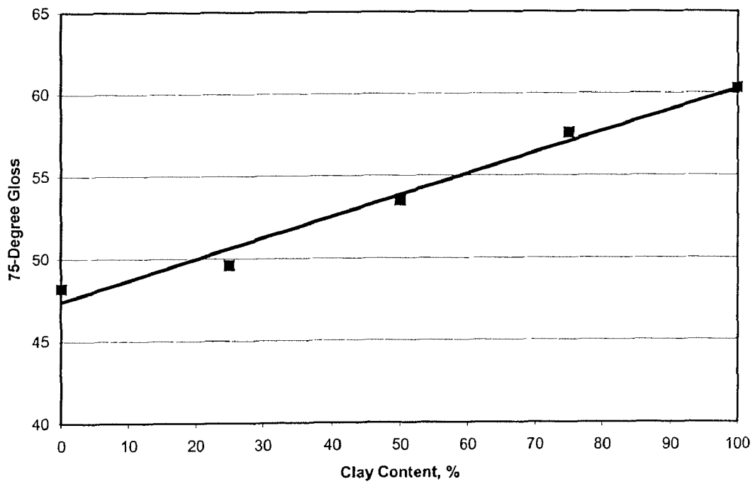
Figure 3. Gloss versus % Kaolin Clay
