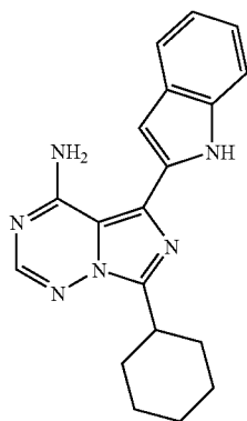
7-Cyclohexyl-5-(1H-indol-2-yl)imidazo [5,1-f][1,2, 4]triazin-4-amine
