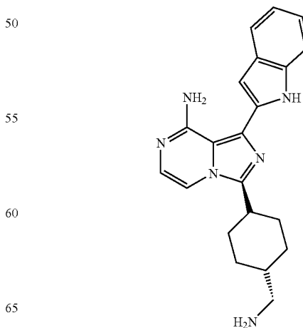
7-Cyclohexyl-5-(1H-indol-2-yl)imidazo [5,1-f][1,2, 4]triazin-4-amine
