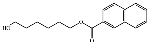
STRUCTURAL FORMULA (I-1)
