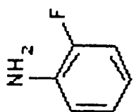
2-Fluoroaniline
