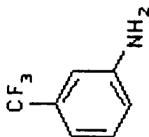
3-Aminobenzotrifluoride
