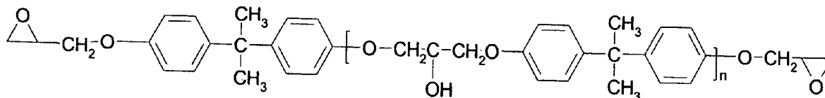
Diglycidylether of Bisphenol-A (DGEBA).
