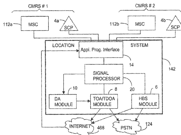
WIRELESS LOCATION USING MULTIPLE CMRSs
