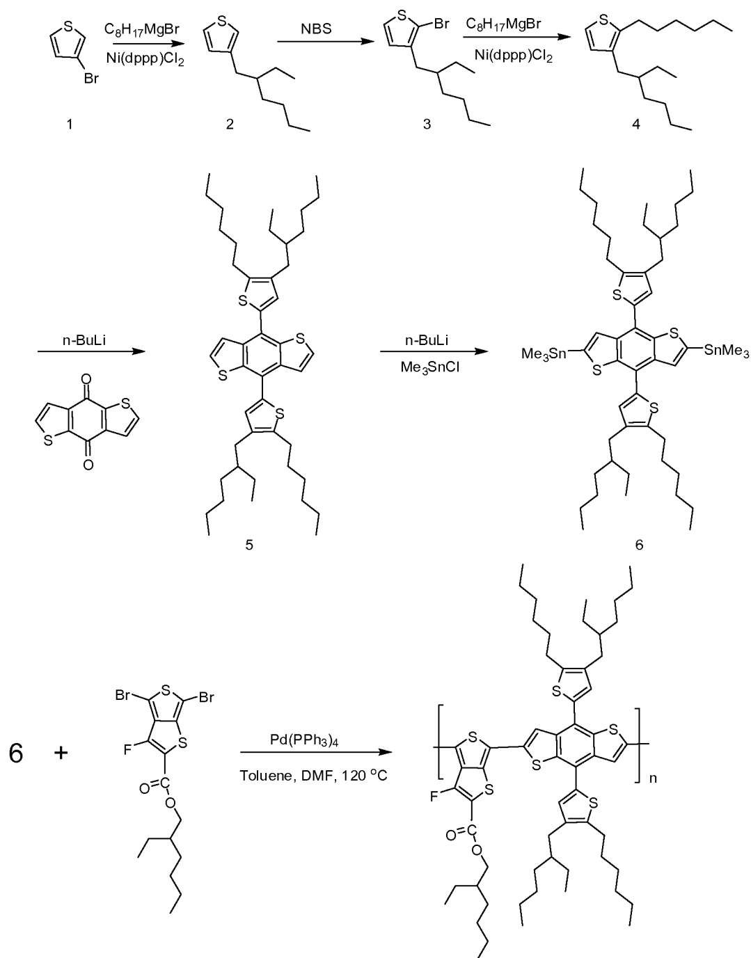
Scheme 4. The synthetic route for monomers and polymers PTBT-X
