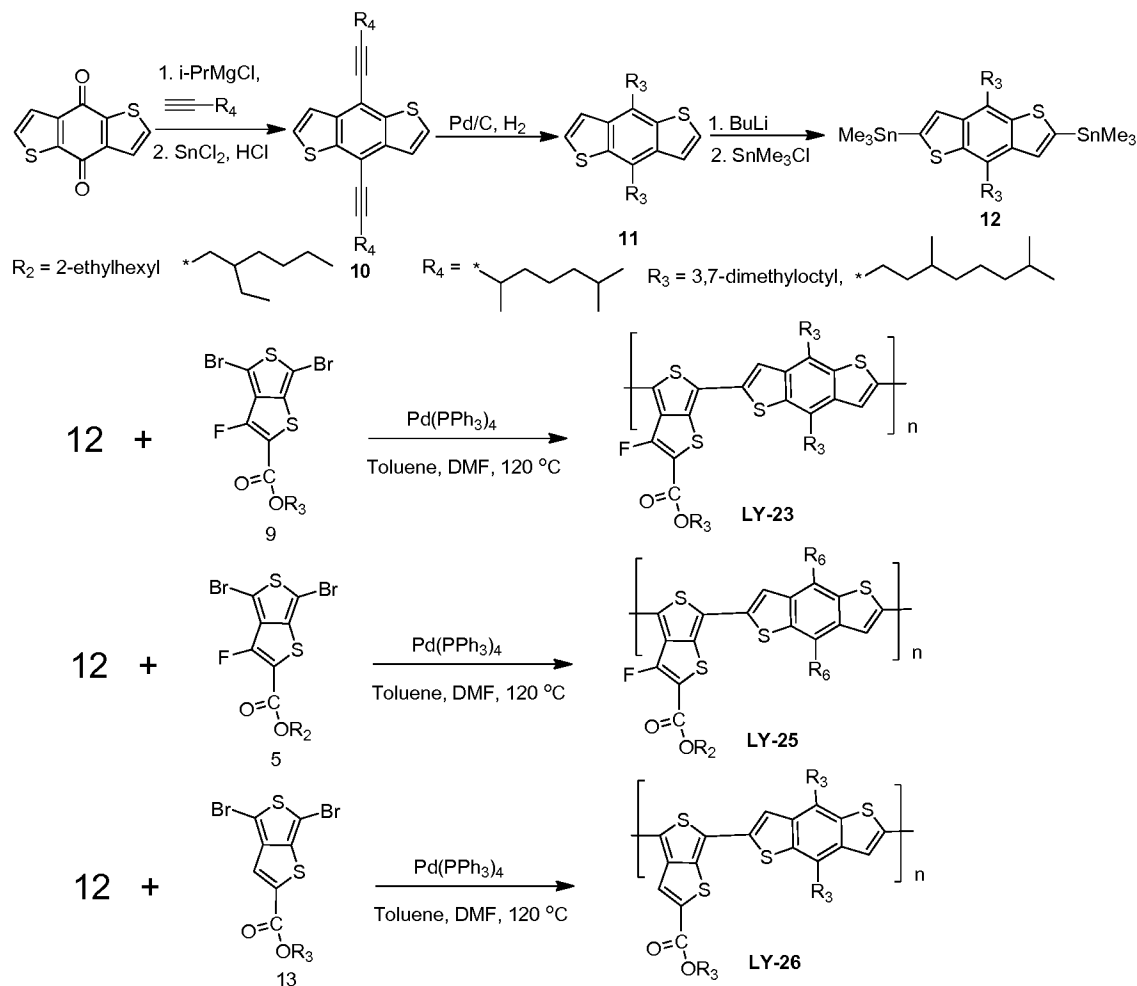
Scheme 3. Synthesis of Polymer LY-23, LY-25 & LY-26.
