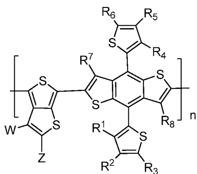
Formula Ia
