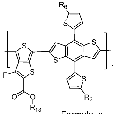
Formula Id
