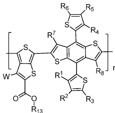
Formula Ib
