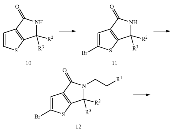
Scheme 4: Synthesis of Compound 1
