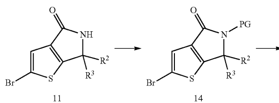
Scheme 5: Alternative synthesis of Compound 1
