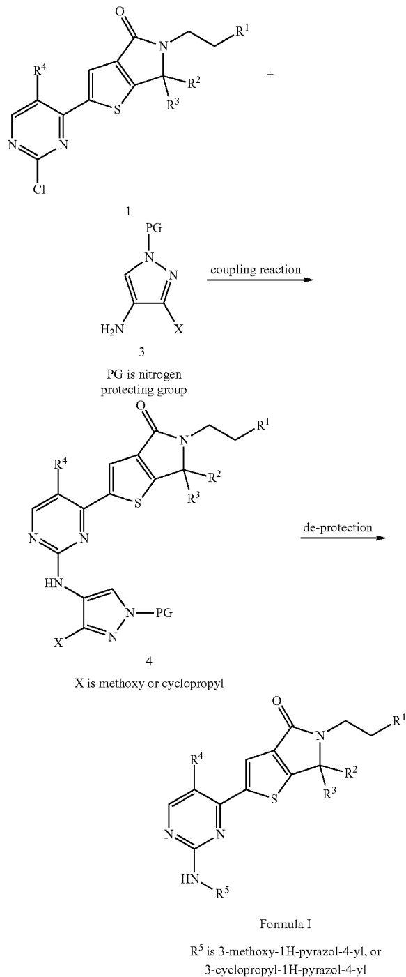
Scheme 2: Synthesis of compounds of Formula I when R 3 is 3-methoxy-1H-pyrazol-4-yl or 3-cyclopropyl-1H-pyrazol-4-yl
