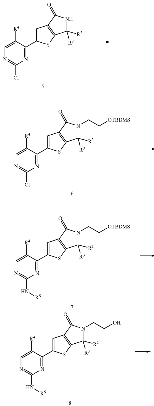
Scheme 3: Alternative synthesis of compounds of Formula I
