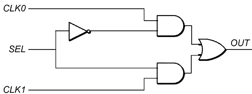
FIG. 8 (Prior Art)
