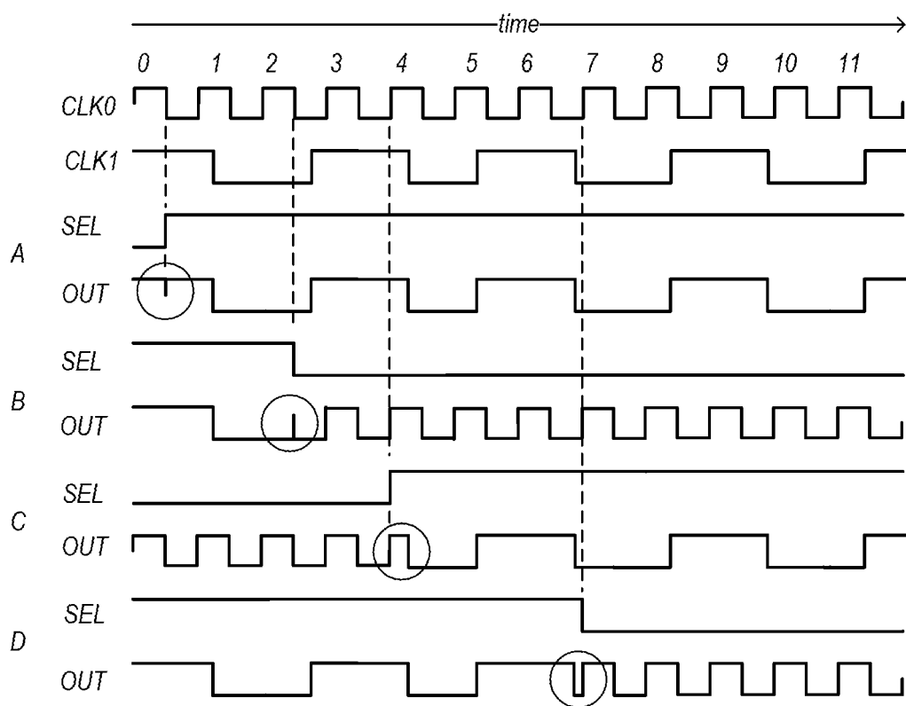
FIG. 9 (Prior Art)
