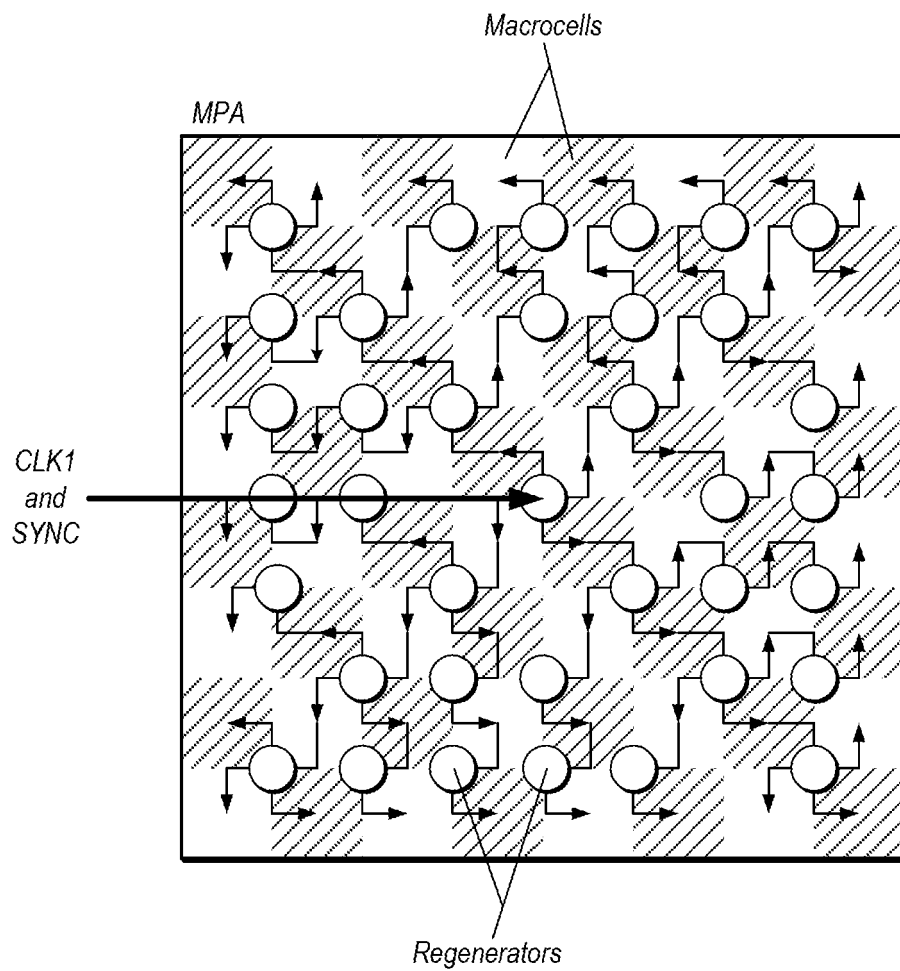
FIG. 2 (Prior Art)
