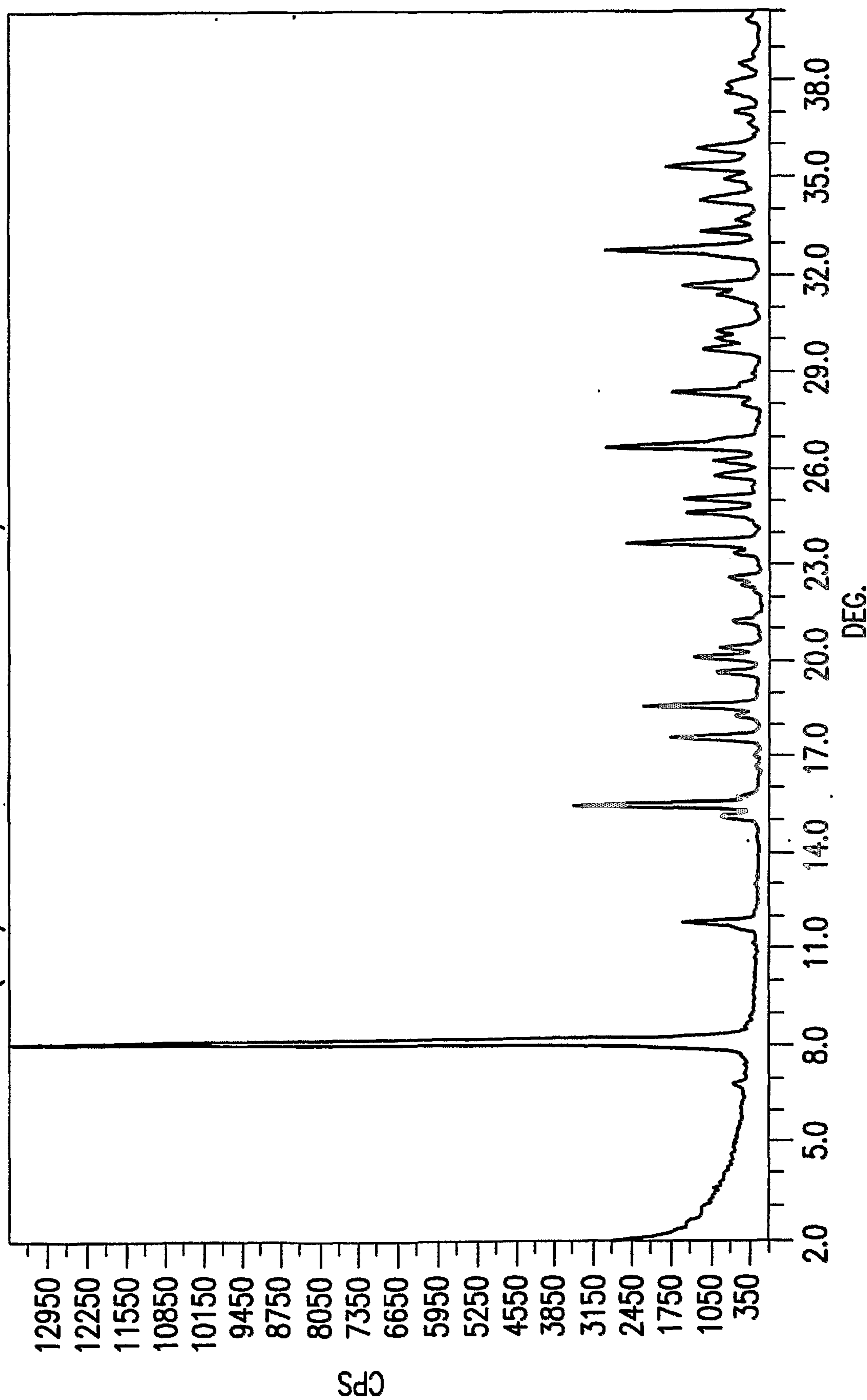
FIG.9 X-RAY POWDER DIFFRACTION OF ZOLEDRONATE MONOSODIUM FORM VIII
