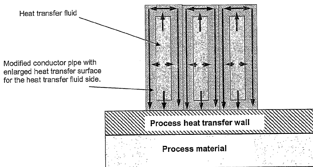
Section through oblong conductor pipes
