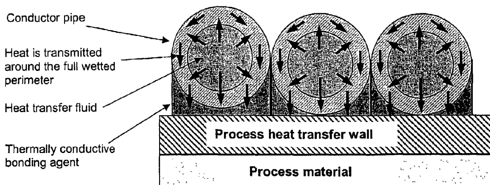
Section showing circular conductor pipes bonded to the heat transfer surface
