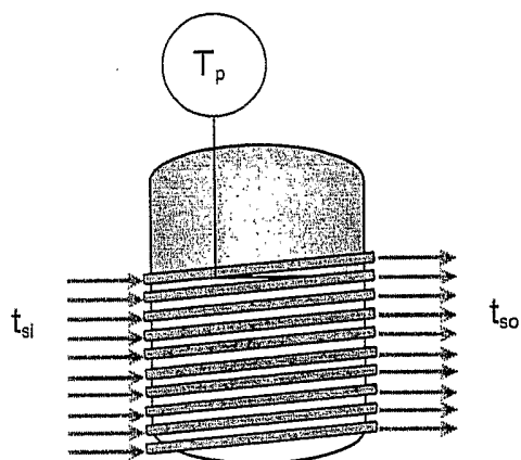
Heat transfer arrangement for a reduced volume jacket
