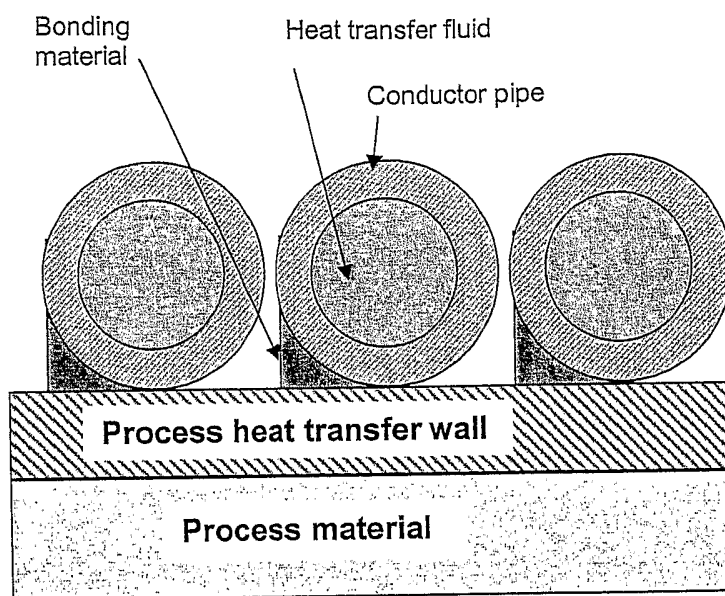
One-sided solder bonding
