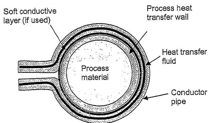
Simple spring mounted conductor pipe
