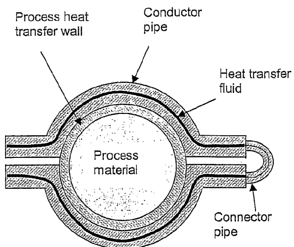
Two part mounted conductor pipe configuration
