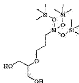
Pendant silicone diol compound 6
