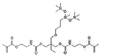
Pendant silicone urethane (meth) acrylate 5
