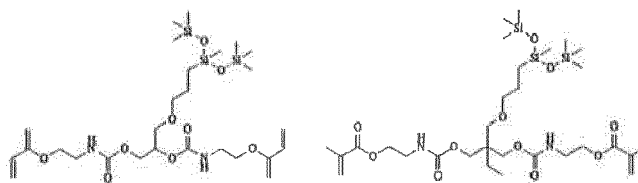
Pendant silicone urethane (meth) acrylate 4
