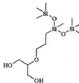
Pendant silicone diol compound 2
