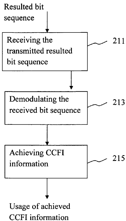
Receiving Flowchart 1
