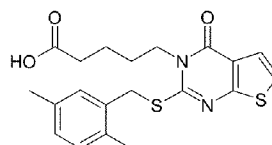
Compound 9
