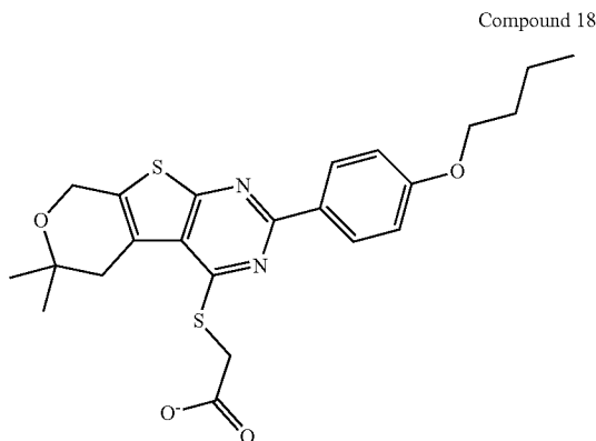
Compound 18
