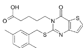
Compound 3
