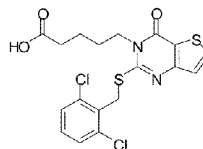
Compound 7
