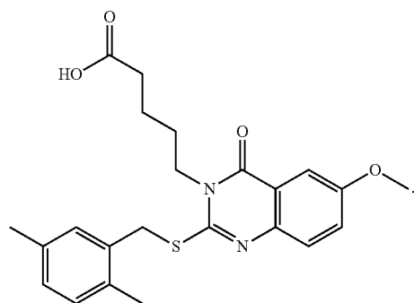
Compound 16
