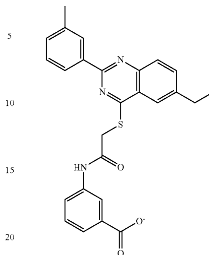
Compound 16
