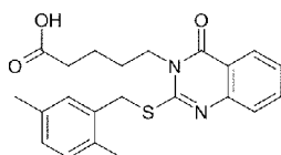
Compound 8
