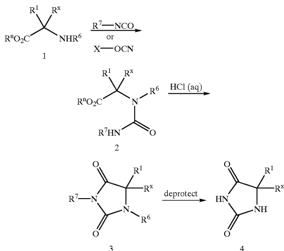
Scheme 1 Heterocycle Synthetic Routes
