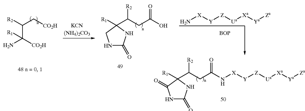
Scheme 8. Amide substituted non-spirocyclic hydantoin
