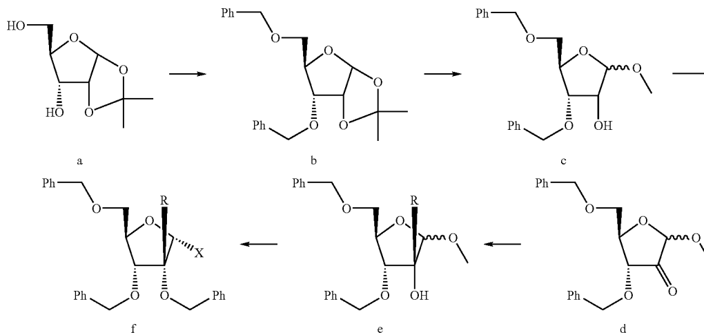
Scheme 1: Alternative Sugar Synthesis and Coupling
