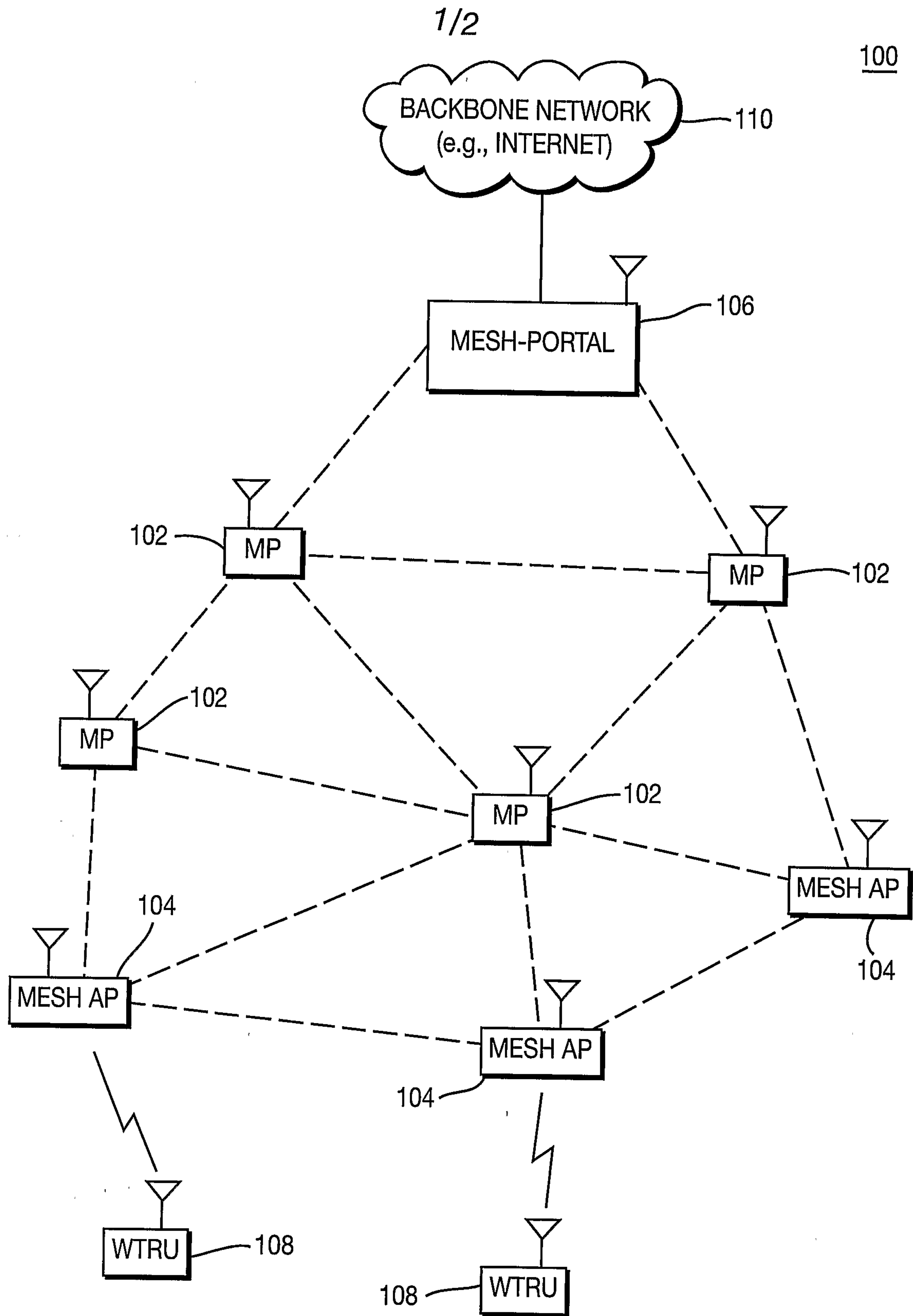
FIG. 1 PRIOR ART
