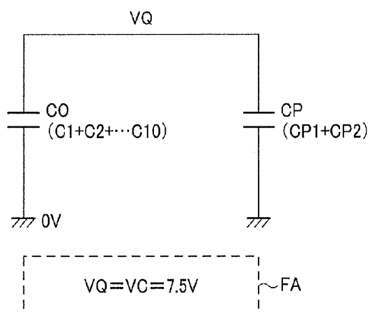
FIG. 2B MAXIMUM DATA VOLTAGE
