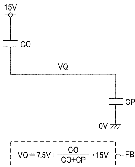
FIG. 2B MAXIMUM DATA VOLTAGE
