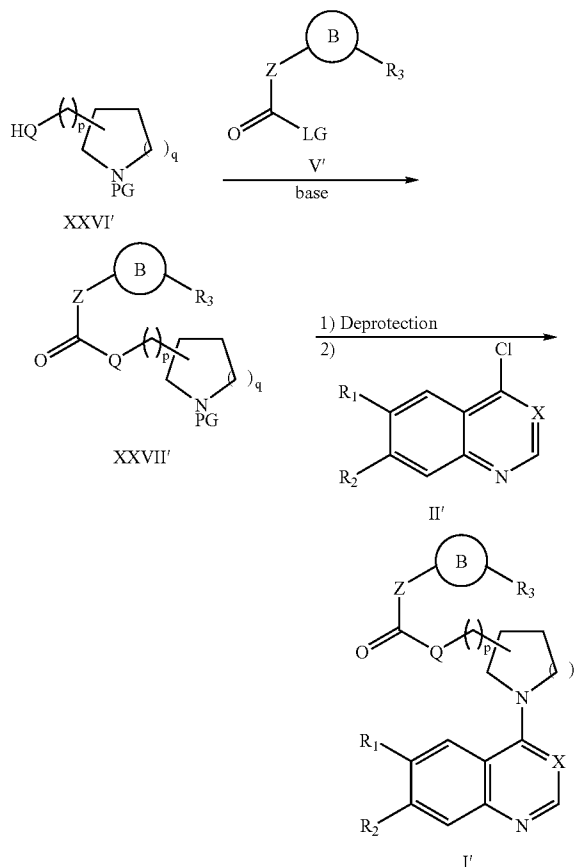
Scheme 12
