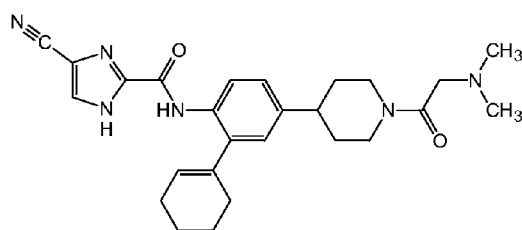
FLT3 Inhibitor Compound D
