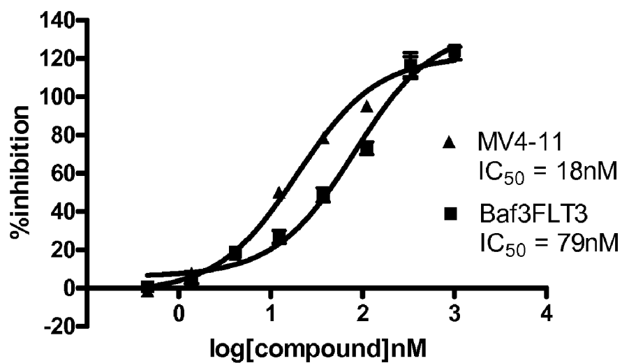
Figure 6.3. Dose responses of Compound C on FLT3-dependent AML cell proliferation
