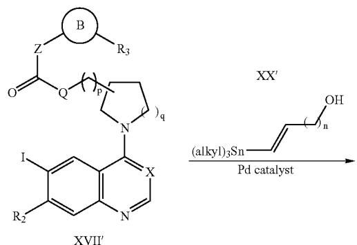
Scheme 9
