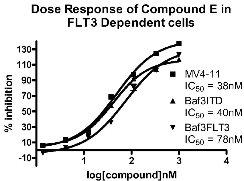
Figure 6.6. Dose responses of Compound E on FLT3-dependent AML cell proliferation
