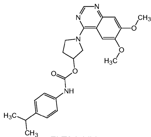
FLT3 Inhibitor Compound H
