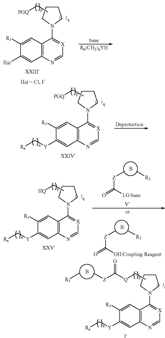
Scheme 11
