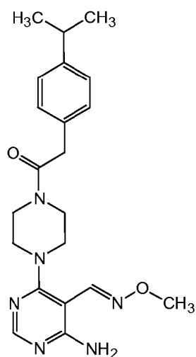
FLT3 Inhibitor Compound F
