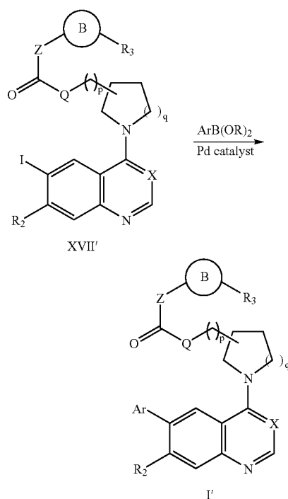
Scheme 10
