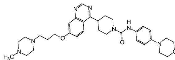
FLT3 Inhibitor Compound B
