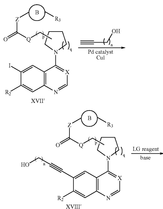
Scheme 8
