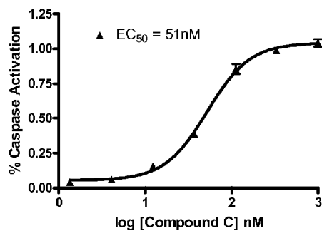
C Dose -Response of Caspase activation by Compound C in MV4-11 cells
