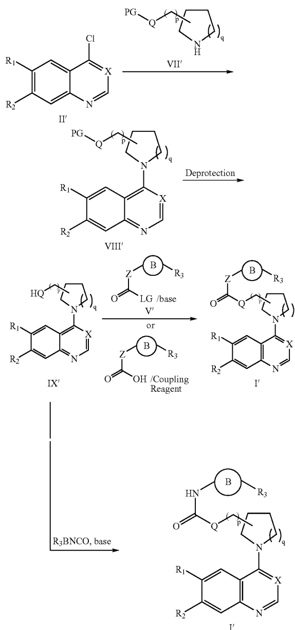
Scheme 4
