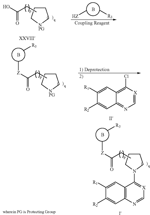
Scheme 13
