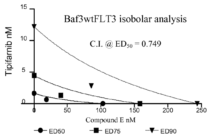
Figure 10.6. Compound E and Tipifarnib synergistically inhibit the proliferation of FLT3-dependent cells as measured by the method of Chou and Talalay
