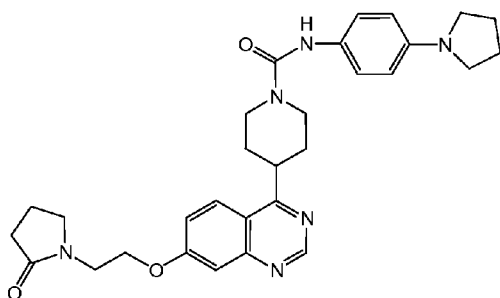
FLT3 Inhibitor Compound C
