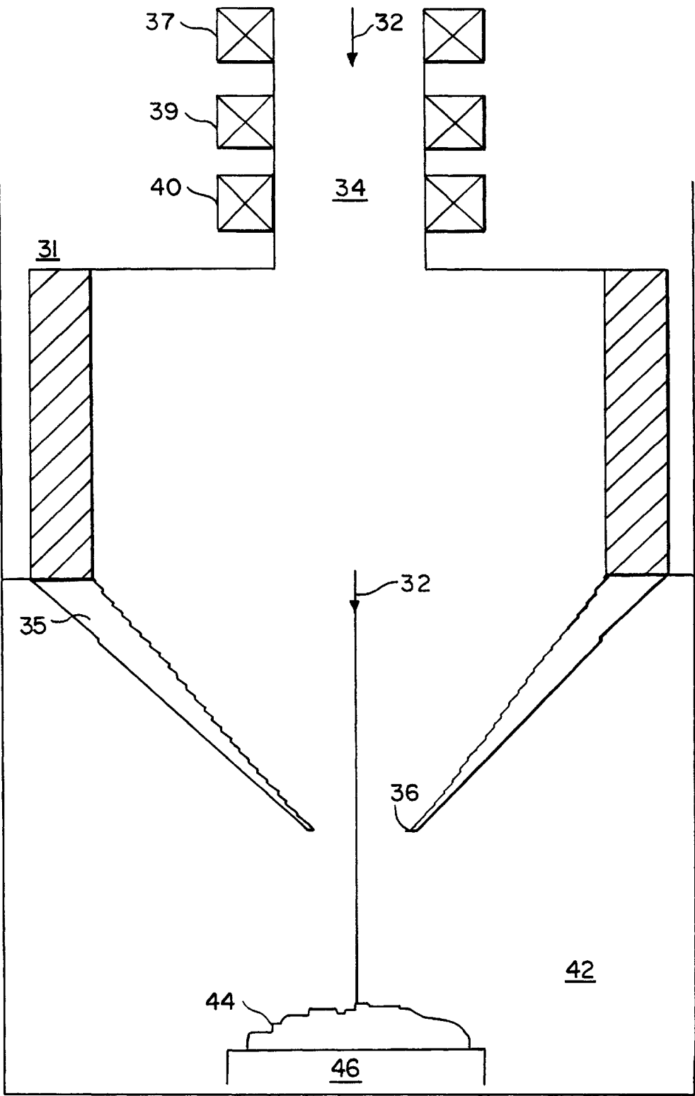
FIG. 2 PRIOR ART
