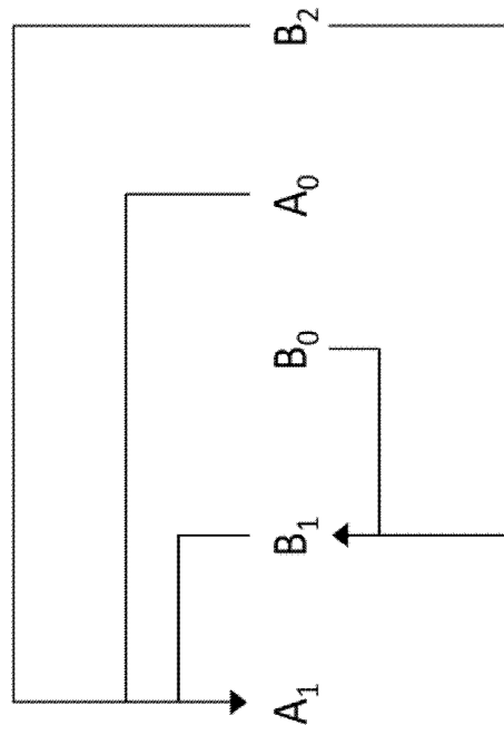
Candidate pairs considered for redundancy check of spatial merge candidates
