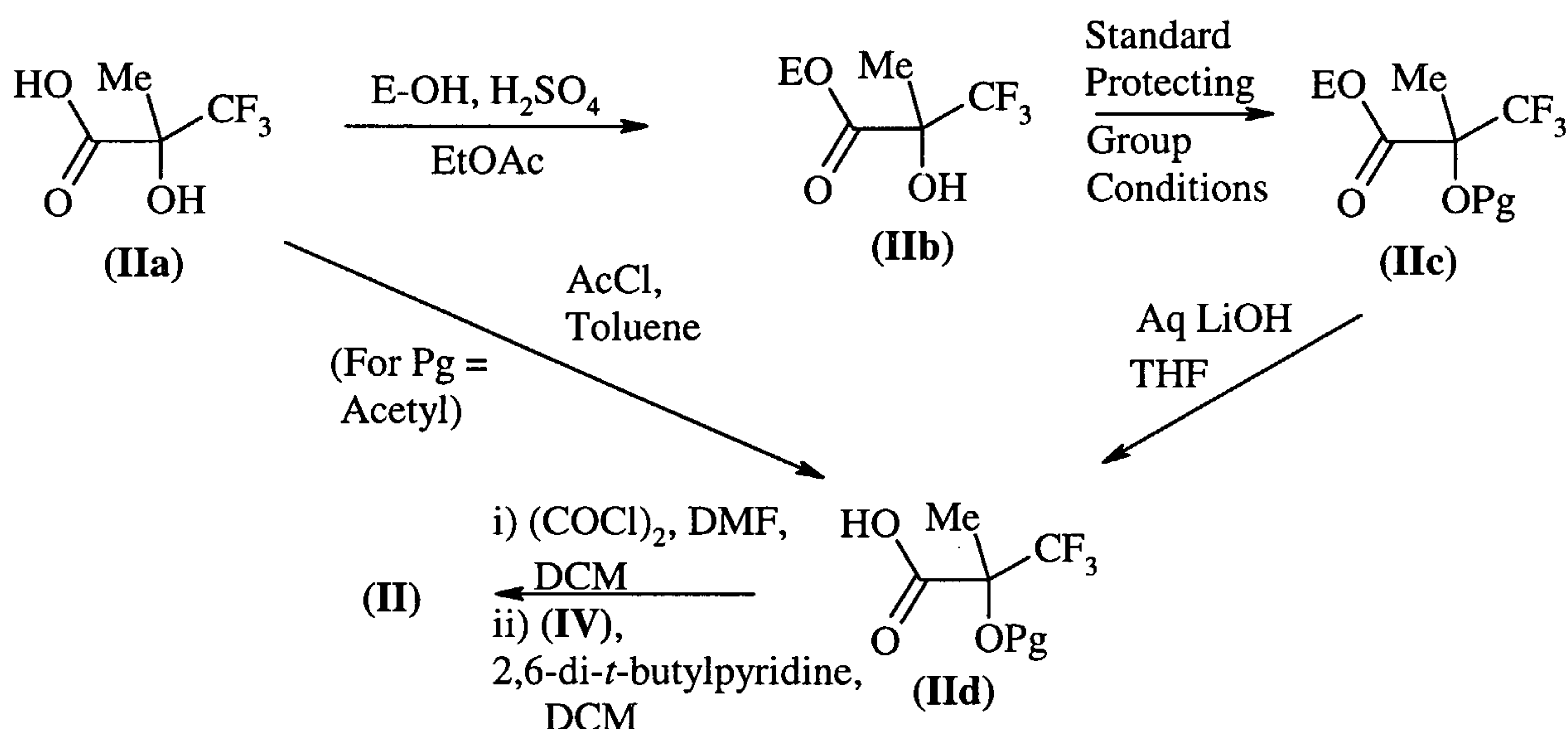
Scheme 1
