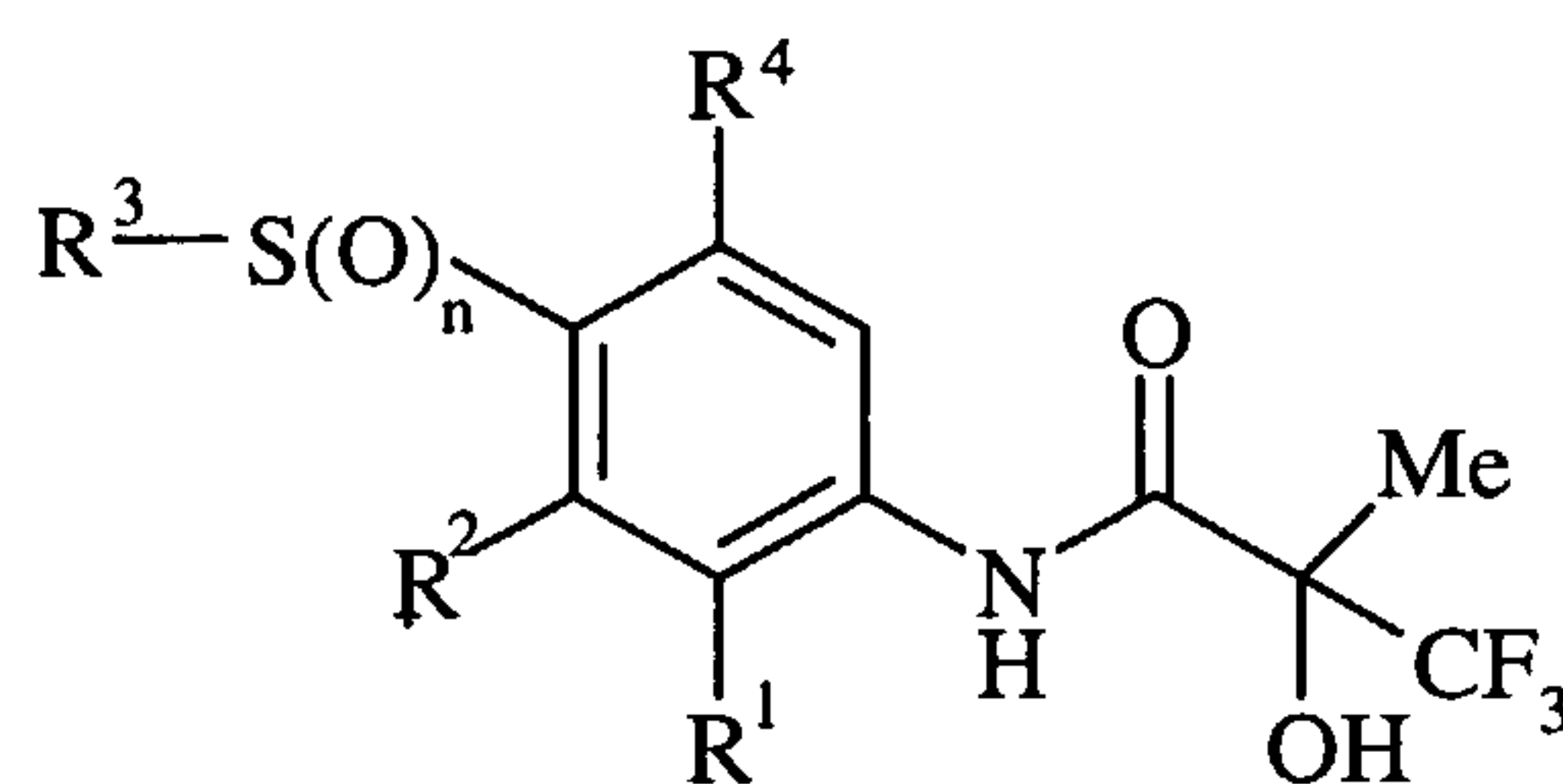
(I)
