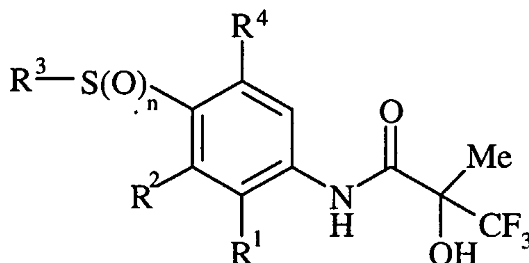
(I)
