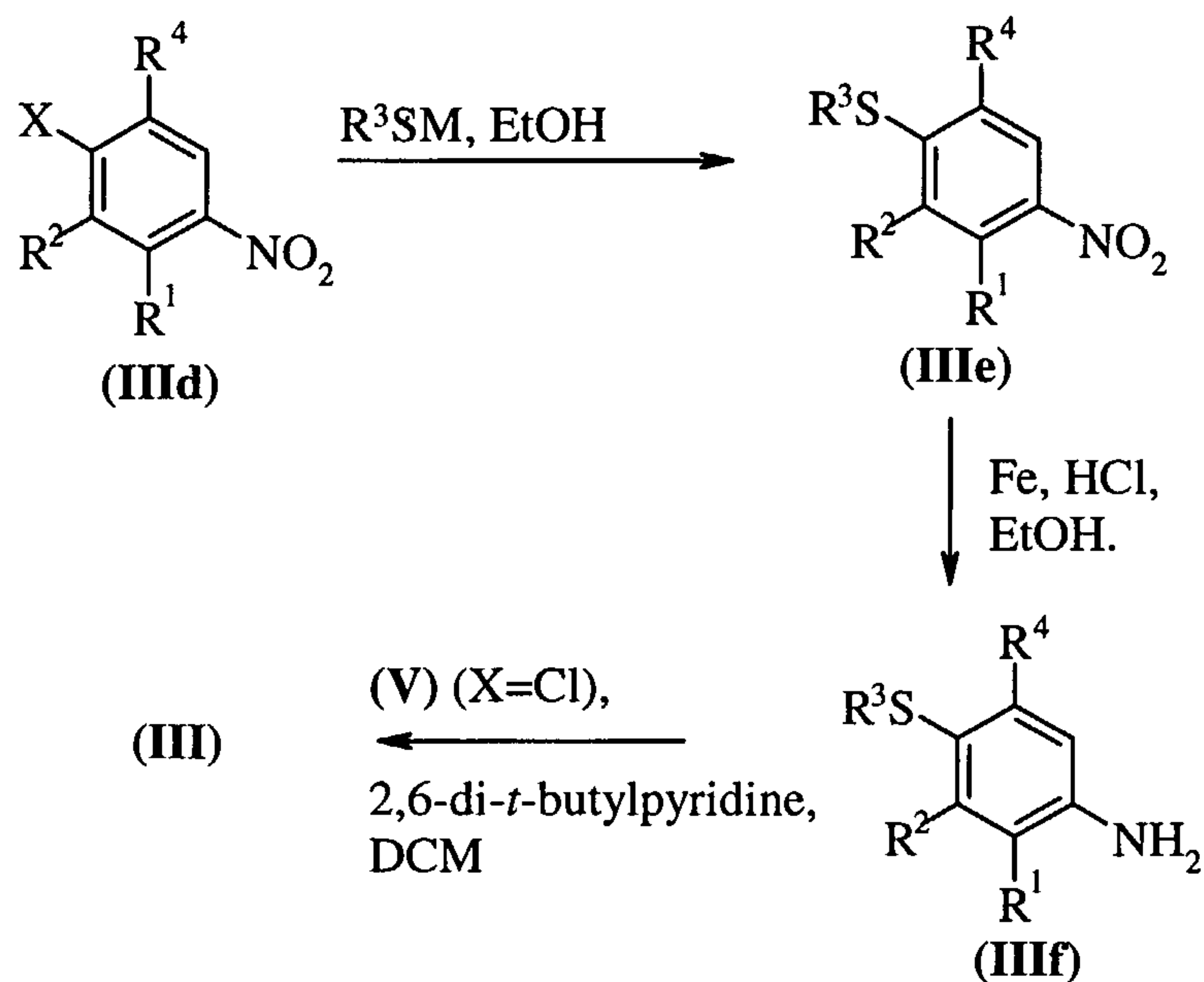
Scheme 3
