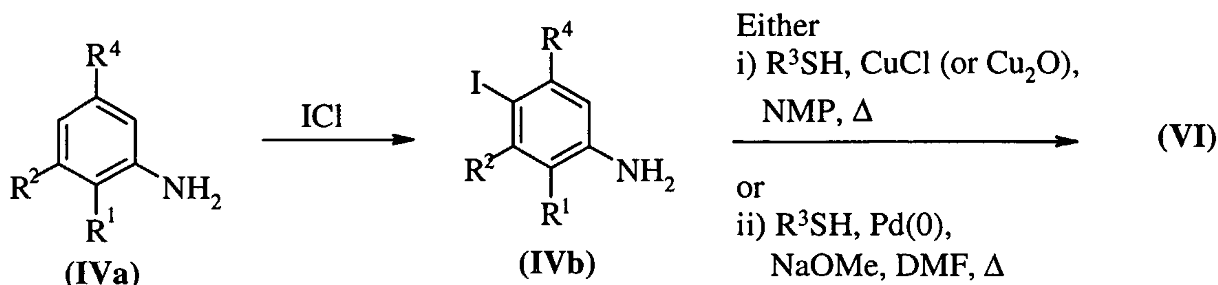
Scheme 5
