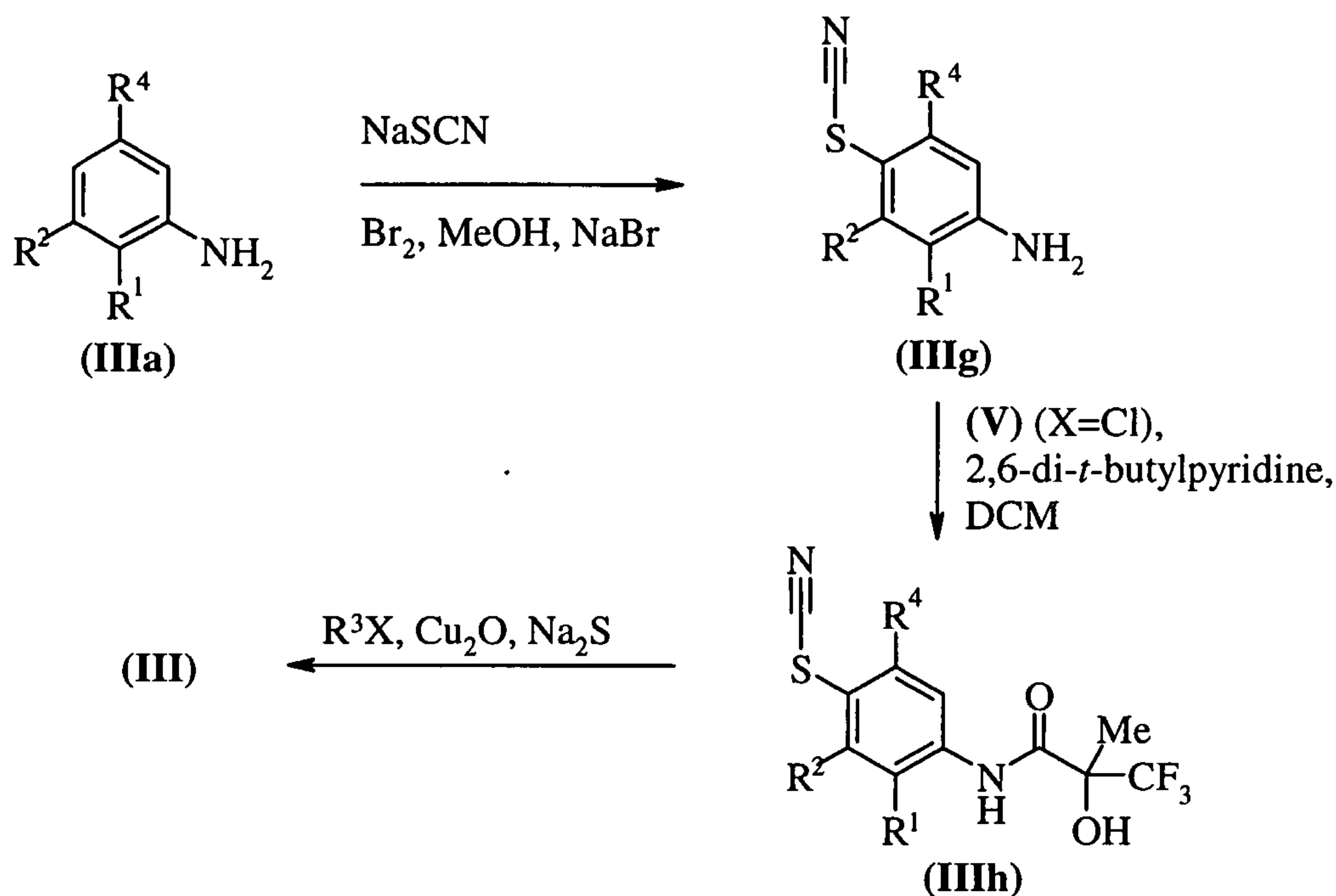
Scheme 4
