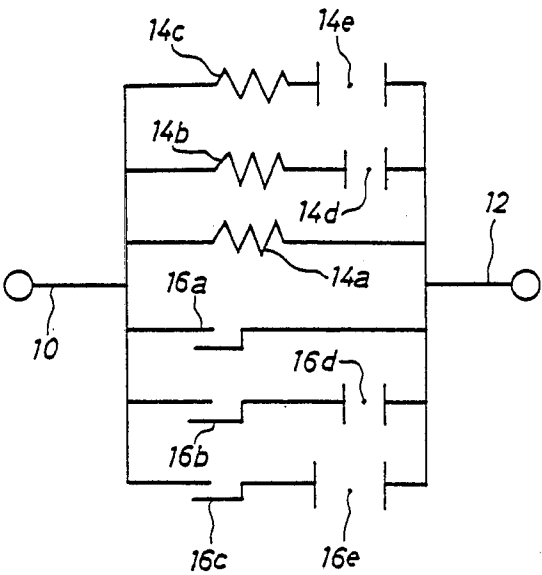
PRIOR ART FIG. 10
