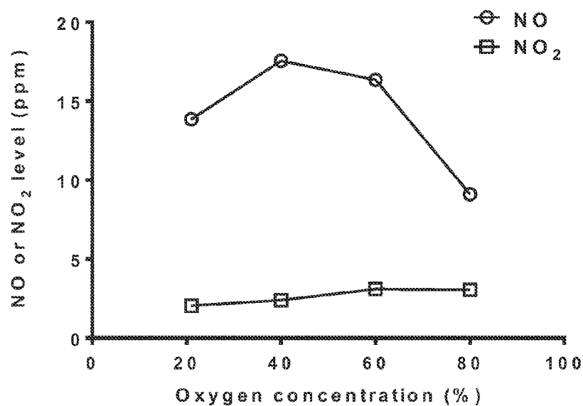
Production of NO and NO 2 at different O 2 levels
