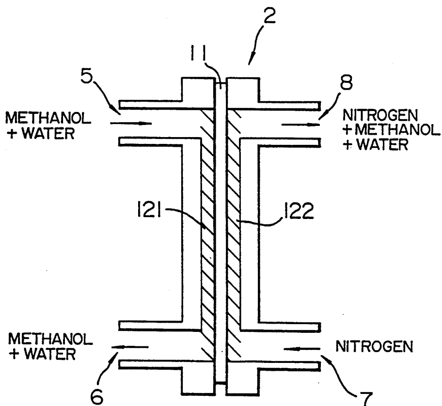
DETAIL VIEW OF A MEASURING CELL
