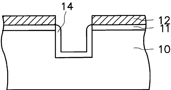
FIG. 1C (PRIOR ART)
