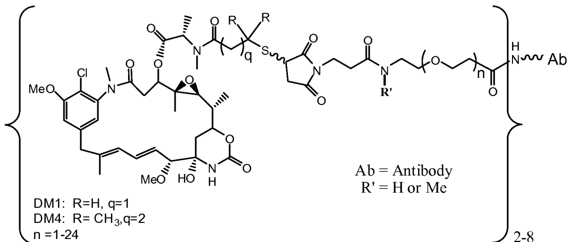
Ab-PEG-Mal-DM1/DM4
