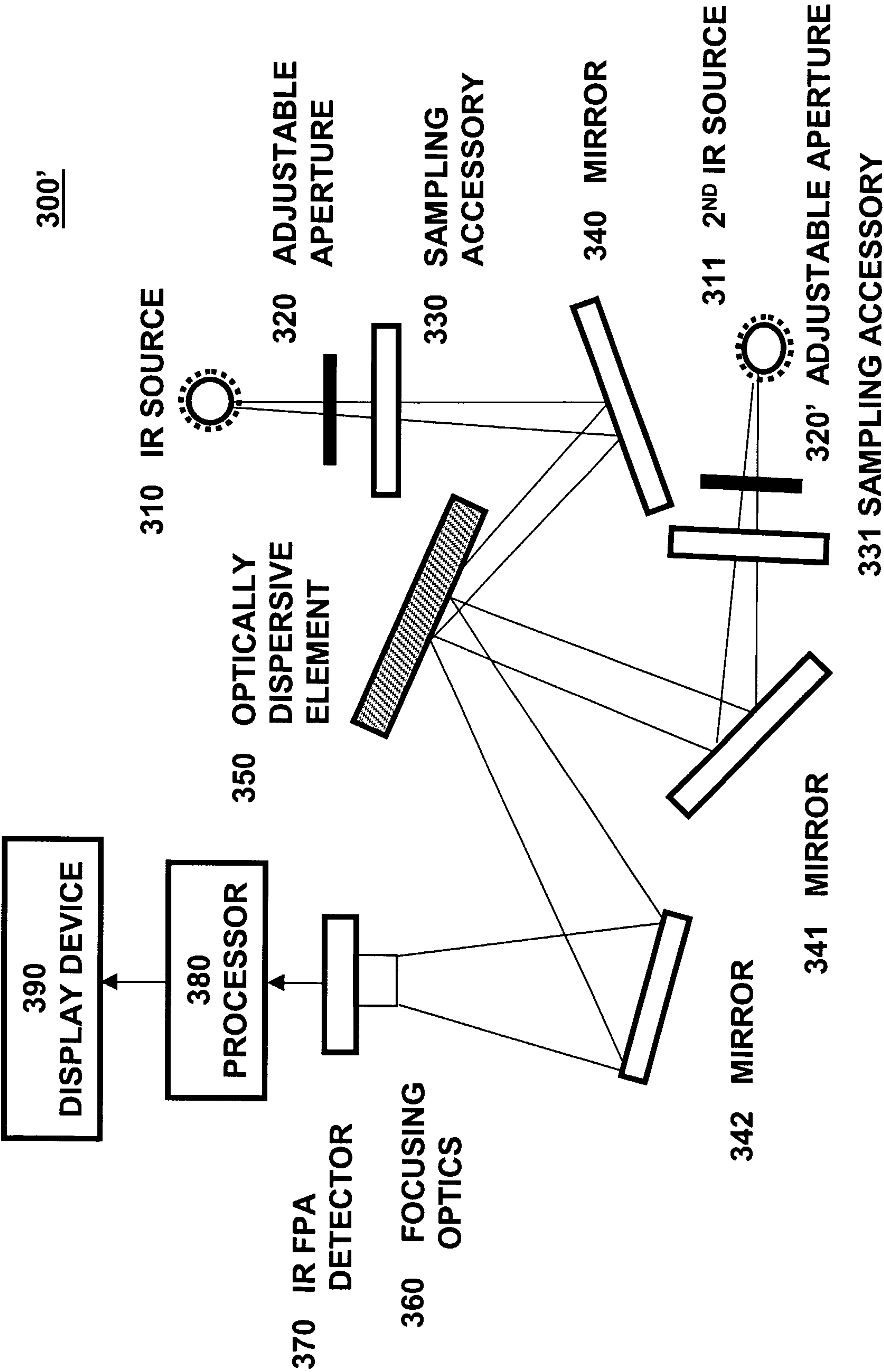
FIG. 3B MULTIPLE SOURCES/SAMPLES
