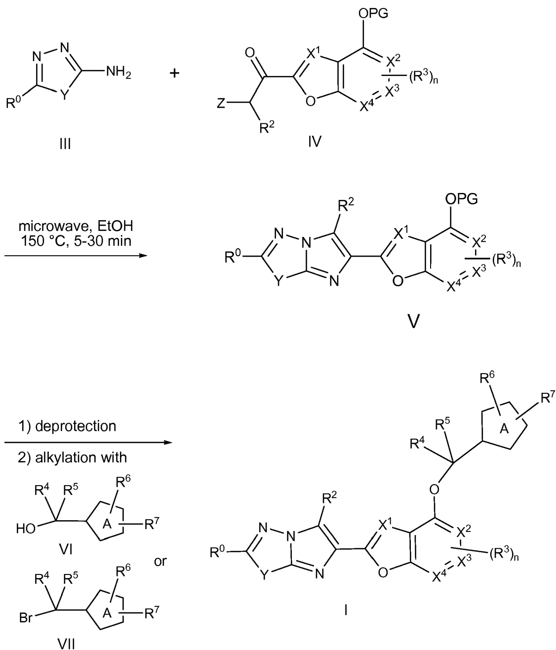
Scheme 1
