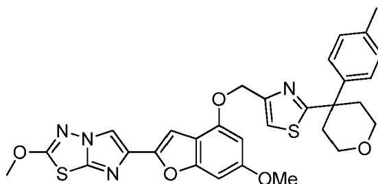
157A. (2-(4-(p-Tolyl)tetrahydro-2H-pyran-4-yl)thiazol-4-yl)methanol
