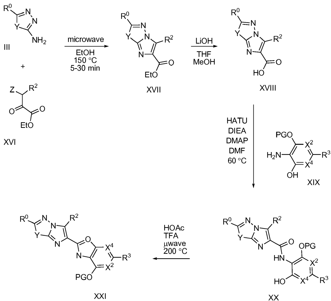
Scheme 4
