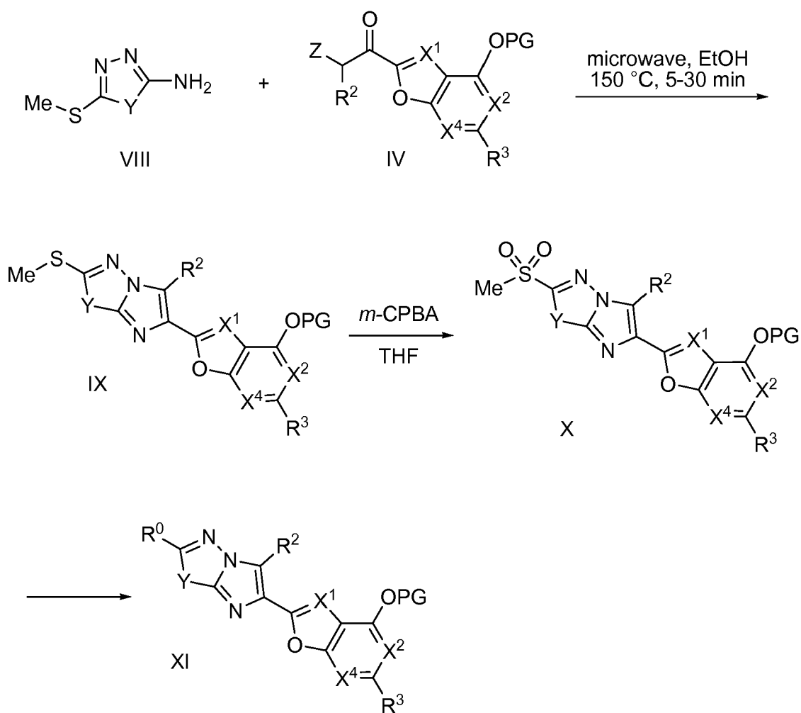
Scheme 2
