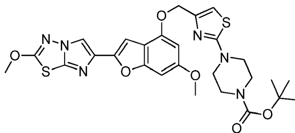
99A. Methyl 2-(4-( tert -butoxycarbonyl)piperazin-1-yl)thiazole-4-carboxylate
